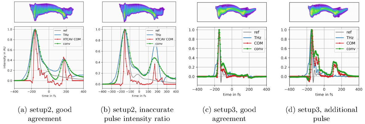
Figure 3: Four single-shot examples. Here, time zero is defined as the horizontal center of mass of the TDS image. The THz streaking curves are shifted accordingly. 'ref' is the photoelectron spectrum without THz streaking field and is convoluted with the TDS profiles to compare both curves with a similar resolution (conv). We see two examples where the methods agree well (a,c), and two where we get an artefact in the analysis (b,d).
