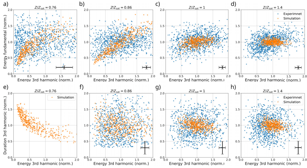
Fig. 5. The upper row shows the experimental and simulated data the for single-shot pulse energy of the fundamental and third harmonic, at different stages of amplification. All shown data is normalized to the respective mean value. The experimental data does not show a correlation. The lower row shows experimental and simulated data for the pulse duration and pulse energy of the third harmonic. In e), the experimental result is not shown since the third harmonic signal was too low for a reliable pulse duration measurement.
