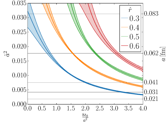
Figure 4: Location of the maximum of \hat{\chi}(\hat{a}) as a function of the smearing strength \frac{8t_0}{a^2} for several distances \hat{r} \equiv \frac{r}{\sqrt{8t_0}} .
