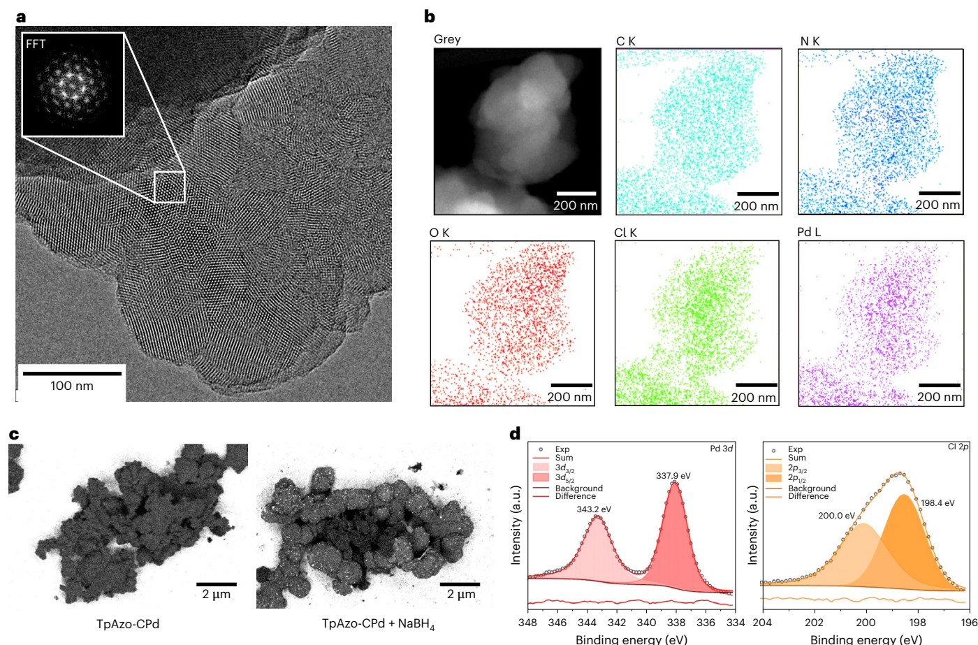
Fig. 5 | Characterization of isolated palladium atoms in TpAzo-CPd COF. a, High-resolution TEM image and fast Fourier transform of a selected area. b, STEM-EDX elemental mapping analysis of the area shown at the top left. c, SEM images using ESB/SE2 detectors. d, Palladium 3d and Cl 2p XPS spectra.
