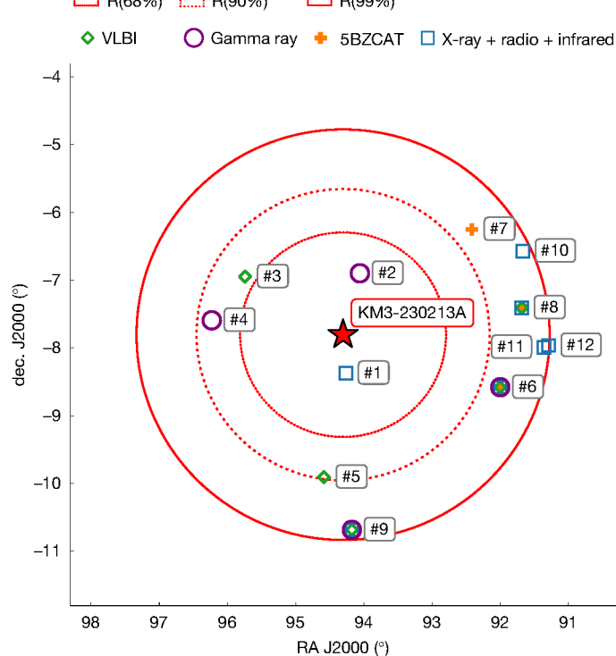
Fig. 4 | Sky map in the direction of KM3-230213A. KM3-230213A is indicated by the red star, with the error regions within R(68%), R(90%) and R(99%) shown as dotted, dashed and solid contours, respectively. The directions of the selected source candidates are shown as coloured markers, whose colours and marker type indicate the criterion according to which the source was selected. The sources are numbered according to their proximity to KM3-230213A, as reported in Methods.
