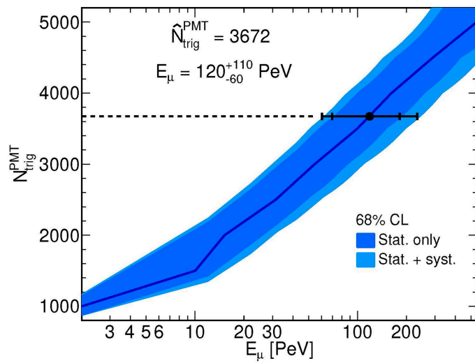
Extended Data Fig. 3 | Energy measurement. Left, the true muon energy E_\mu maximizing the likelihood value for a given \mathcal{N}_{\text{trig}}^{\text{PMT}} is shown as a blue line. The blue bands show the 1\sigma confidence level, computed from the likelihood distribution using Wilks' theorem 13 : in dark blue when only statistical uncertainties are considered, in light blue when systematic uncertainties are also included. The observed value \hat{\mathcal{N}}_{\text{trig}}^{\text{PMT}} = 3,672 corresponds to the horizontal
