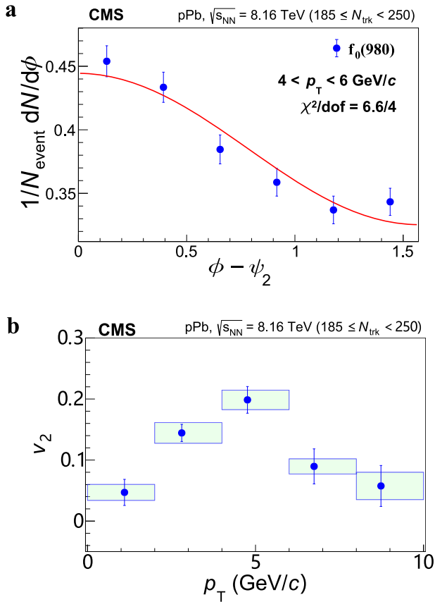
Fig. 6 | Elliptic anisotropy before the nonflow effect subtraction. a The f_0(980) yield in the 4 < p_T < 6 GeV/c range as a function of \phi - \psi_2 in high-multiplicity pPb collisions. Error bars show statistical uncertainties. The red curve is a fit to Eq. (1) with only the n = 2 term, from which the elliptic anisotropy v_2 parameter is extracted. b The elliptic anisotropy v_2 of the f_0(980) state is shown before the nonflow effect subtraction as a function of p_T within rapidity |\eta| \lesssim 2.4 in high-multiplicity pPb collisions. The error bars show statistical uncertainties while the shaded areas represent systematic uncertainties.
