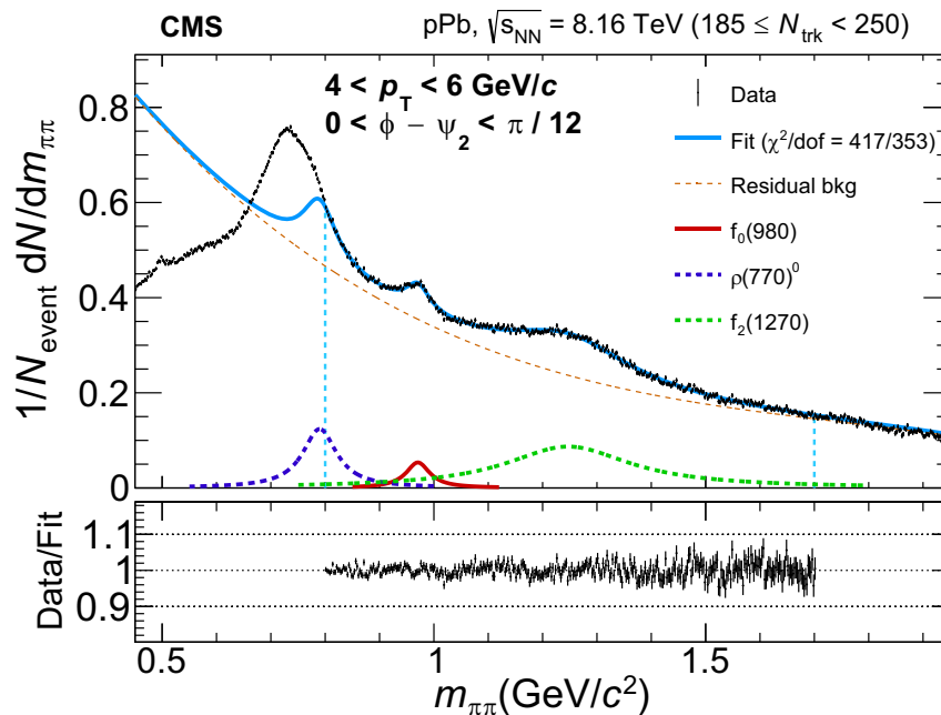
Fig. 5 | Invariant mass fit. The invariant mass spectrum of opposite-sign pion pairs after the combinatorial background subtraction, for the pair transverse momentum 4 < p_T < 6 GeV/c and the azimuthal angle 0 < \phi - \psi_2 < \pi/12 , in high-multiplicity pPb collisions. The solid blue curve is the fit result within the fit range marked with vertical blue dashed lines; the orange dashed curve represents the residual background. The solid red curve represents the f_0(980) signal, while the dashed dark-
