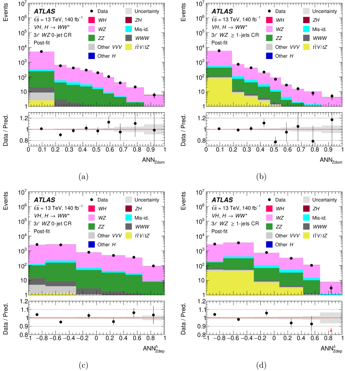
Figure 10. Post-fit distributions of ANN_{Zdom} in the (a) WZ CR with no jets and (b) WZ CR with at least one jet and of ANN_{Zdep}^A in the (c) WZ CR with no jets and (d) WZ CR with at least one jet. The binning of each distribution matches that used in the corresponding SR where that distribution is relevant. The lower panel shows the ratio of the data to the sum of the fitted signal and background, and the arrow in (d) indicates the position of a point outside the vertical axis range. The hatched band shows the total uncertainty. The post-fit results are obtained from the combined 2-POI fit described in section 9.1.
