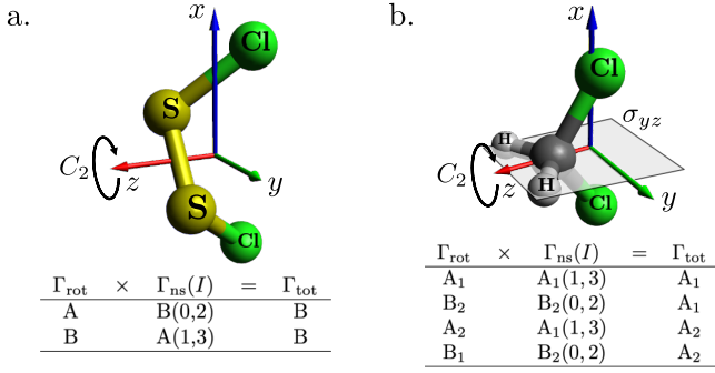
FIG. 1. Equilibrium structures of \text{S}_2\text{Cl}_2 with \text{C}_2 symmetry (a) and \text{CH}_2\text{Cl}_2 with \text{C}_{2v} symmetry (b) in the principal axes system oriented according to the I^r convention, where the a , b , and c axes are assigned to the z , x , and y , respectively. Also shown are the symmetry products used to construct the total spin-rotational wavefunctions, where rotational representations \Gamma_{\text{rot}} are combined with chlorine nuclear spin representations \Gamma_{\text{ns}}(I) for I = 0, 1, 2, 3 , and only products yielding total representations \Gamma_{\text{tot}} that satisfy the Pauli exclusion principle are retained.
