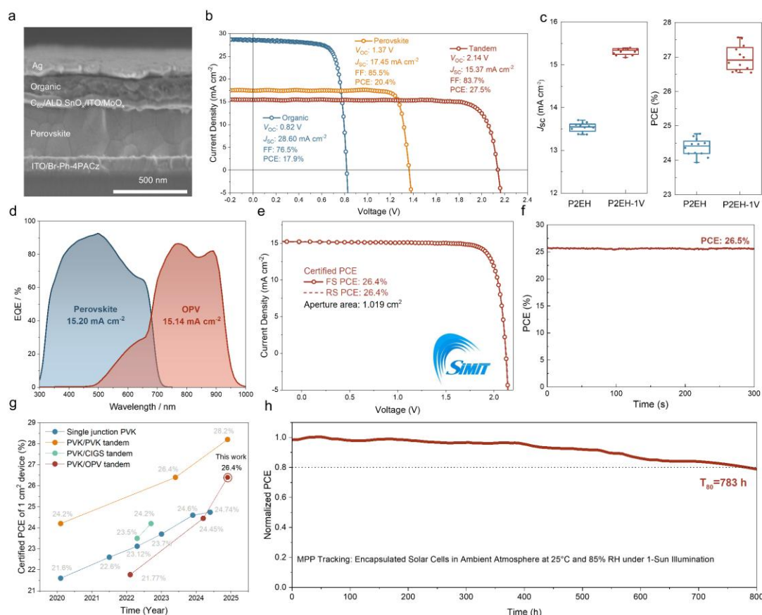
Fig. 4 | Perovskite-organic tandem cells with P2EH-1V and Br-Ph-4PACz. a , Cross-sectional SEM images of perovskite-organic tandem cells. b , Combination of champion J-V curves and photovoltaic parameters of single-junction OPV, perovskite solar cells and perovskite-organic tandem cells. c , Statistical distributions of J sc (left) and PCE (right) of perovskite-organic tandem cells with different NFAs (12 devices for each type). d , EQE curves and integrated J sc for perovskite and organic subcell in perovskite-organic tandem cells, respectively. e , J-V curves of the best 1 cm 2 perovskite-organic tandem cells certified by SIMIT. f , MPP tracking measurement of champion 1 cm 2 device. g , Summary of the reported, independently certified PCEs of centimeter-scale single-junction perovskite solar cells, perovskite-perovskite tandem cells, perovskite-CIGS tandem cells and perovskite-organic tandem cells. h , Long-term MPP tracking results of perovskite-organic tandem cells.
