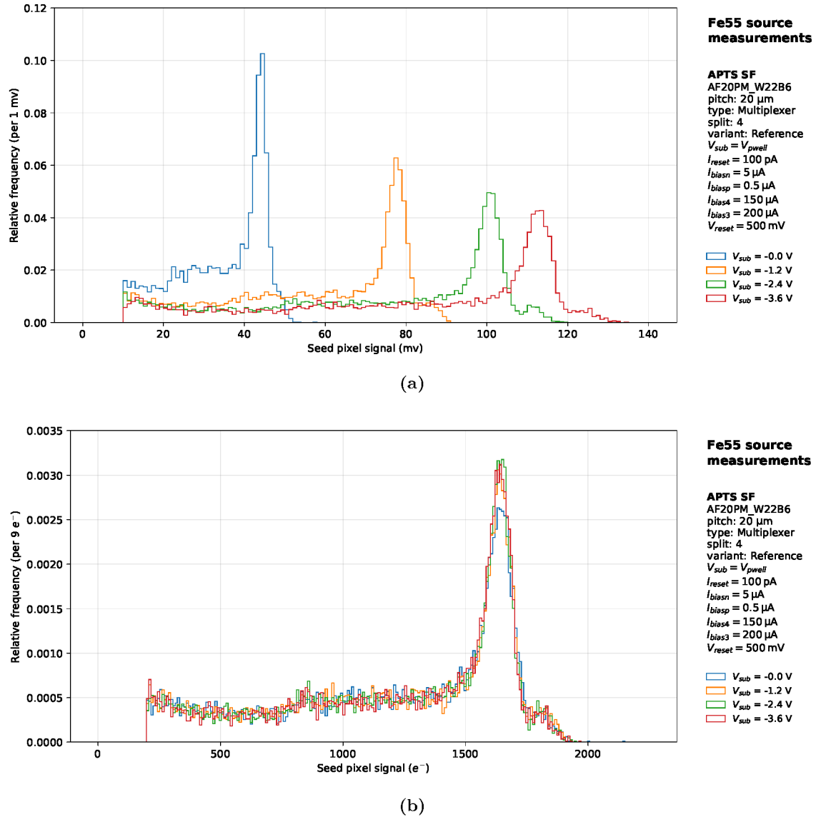
Figure 11.9: ^{55}\text{Fe} seed signal distribution comparing the four different reverse substrate voltages. The reference variant of the APTS-MUX chip with pixel pitch size of 20\mu\text{m} .
