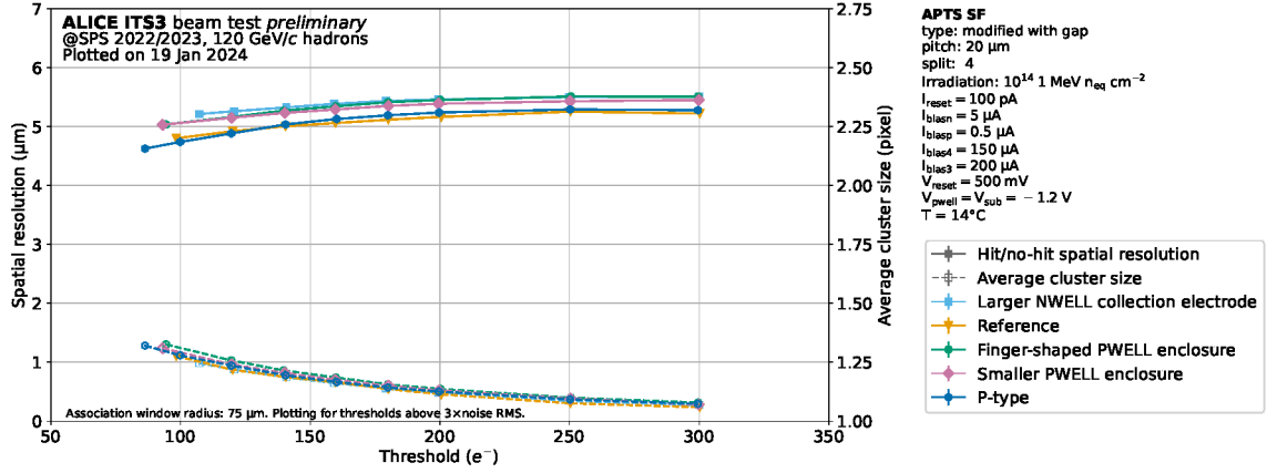
Figure 12.23: The hit/no-hit spatial resolution and the average cluster size as a function of the applied seed threshold, comparing different pixel geometry variants, irradiated to 10^{14} 1 \text{ MeV } n_{\text{eq}} \text{ cm}^{-2} . The first points of measurement correspond to the threshold equivalent to 3 times the noise RMS value. The measurements shown are for the APTS with a pixel pitch size of 20 \mu\text{m} in the ‘Modified with Gap’ process, at the reverse substrate voltage of 1.2 \text{ V} .
