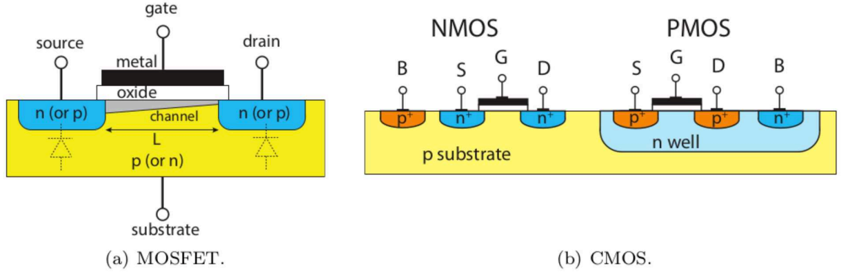
Figure 9.7: The cross-section of (a) a basic MOSFET structure and (b) the realisation of an NMOS and PMOS transistors on the same substrate, also called CMOS. [179]
