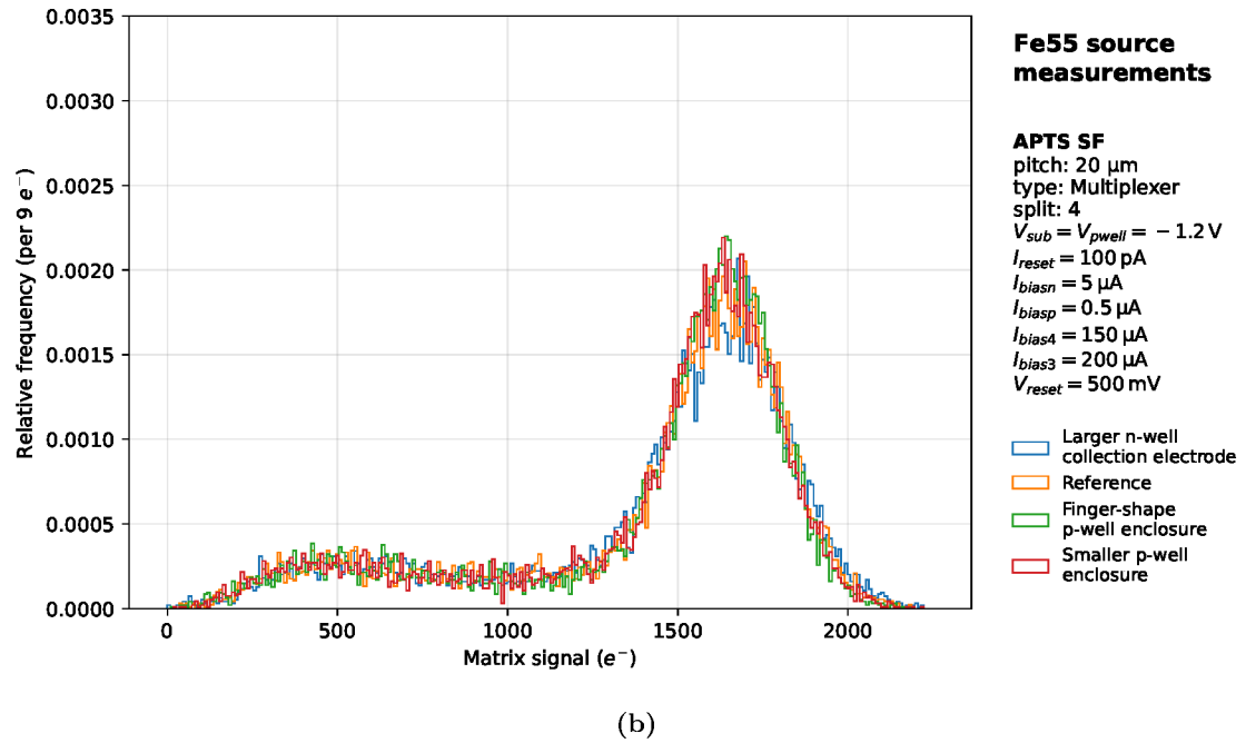
Figure 11.11: ^{55}\text{Fe} matrix signal distribution comparing the four pixel geometry variants. The APTS-MUX chip with pixel pitch size of 20 \mu\text{m} and reverse substrate voltage of 1.2 \text{ V} .
