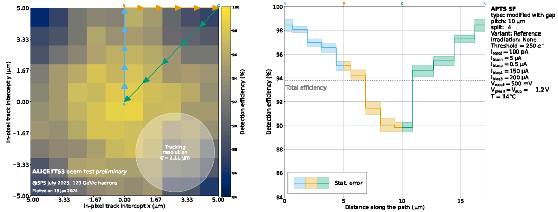
Figure 12.16: The in-pixel detection efficiency at the seed threshold value of 250\ e^- . The left figure shows a single pixel divided into a grid of 10 \times 10 bins, each representing the local detection efficiency. The right figure shows the efficiency along the path within the pixel, as marked in the left figure. The blue histogram indicates the efficiency while moving from the center of the pixel, Point A, to the edge, Point B. the orange histogram illustrates the efficiency while moving along the edge to the corner of the pixel, Point C. And the green path indicates the efficiency while moving from the corner, Point C, back to the center, Point A. The measurements shown correspond to the reference pixel geometry variant APTS with a pixel pitch size of 10\ \mu\text{m} in the ‘Modified with Gap’ process, at the reverse substrate voltage of 1.2\ \text{V} .
