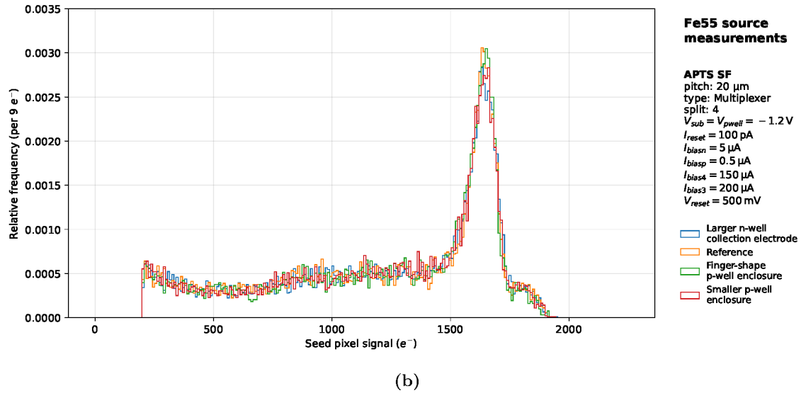
Figure 11.10: ^{55}\text{Fe} seed signal distribution comparing the four pixel geometry variants. The APTS-MUX chip with pixel pitch size of 20\text{ }\mu\text{m} and reverse substrate voltage of 1.2\text{ V} .
