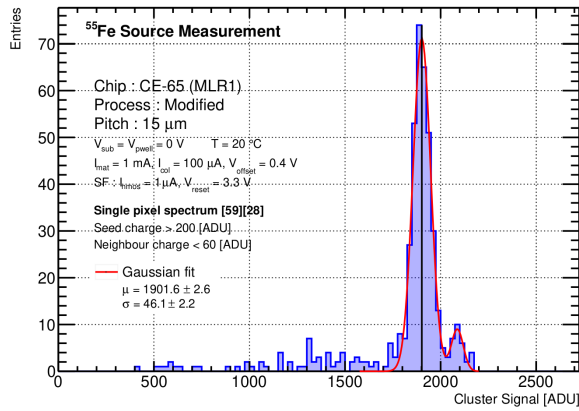
Figure 9.17: The ^{55}\text{Fe} spectrum for single-pixel clusters for an individual pixel ( x = 59, y = 28 ) of the SF submatrix of the CE-65v1 chip in the Modified process with a 15\ \mu\text{m} pitch (a) and for an individual pixel ( x = 20, y = 20 ) of the DC submatrix in the Standard process with a 25\ \mu\text{m} pitch (b). The Gaussian fit is marked in red.
