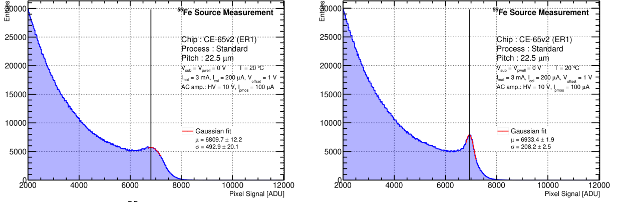
Figure 9.27: The ^{55}\text{Fe} spectrum of the pixel signal after CDS of the entire matrix of the CE-65v2 chip in the Standard process with a 22.5\,\mu\text{m} pitch. The pixel spectrum is shown before (a) and after (b) gain normalisation. The Gaussian fit is marked in red.
