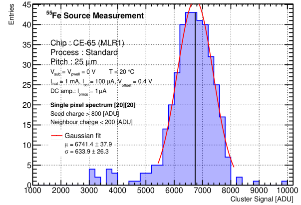
Figure 9.17: The ^{55}\text{Fe} spectrum for single-pixel clusters for an individual pixel ( x = 59, y = 28 ) of the SF submatrix of the CE-65v1 chip in the Modified process with a 15\ \mu\text{m} pitch (a) and for an individual pixel ( x = 20, y = 20 ) of the DC submatrix in the Standard process with a 25\ \mu\text{m} pitch (b). The Gaussian fit is marked in red.
