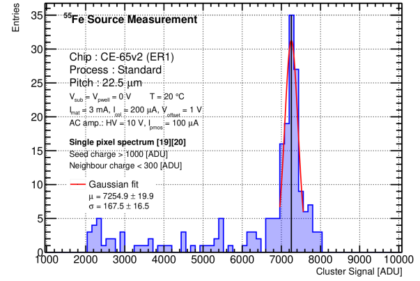
Figure 9.16: The ^{55}\text{Fe} spectrum for single-pixel clusters for an individual pixel ( x = 5, y = 2 ) of the CE-65v2 chip in the Modified with Gap process with a 15\ \mu\text{m} pitch (a). ^{55}\text{Fe} spectrum for single-pixel clusters for an individual pixel ( x = 19, y = 20 ) of the CE-65v2 chip in the Standard process with a 22.5\ \mu\text{m} pitch (b). The Gaussian fit is marked in red.
