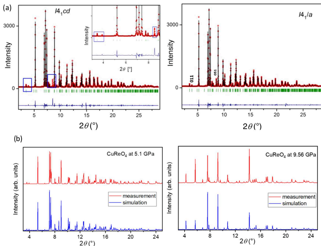
Figure 4. (a) Diffraction patterns of CuReO 4 -HP(I) at 1.73 GPa with the experimental (red), theoretical (black, Le Bail refinement), and differential (blue) curves, analyzed using I4_1cd and I4_1/a space groups. Two notable Bragg reflections, 011 and 051 at 2\theta = 3.9 and 8.7^\circ , respectively, are inconsistent with the I4_1cd space group (left) and indicate the I4_1/a space group (right). (b) Experimental (red) and calculated (blue) diffraction patterns of CuReO 4 -HP(I) at 5.1 GPa and of CuReO 4 -HP(II) at 9.56 GPa. The calculated curves are based on the atomic positions obtained from DFT.
