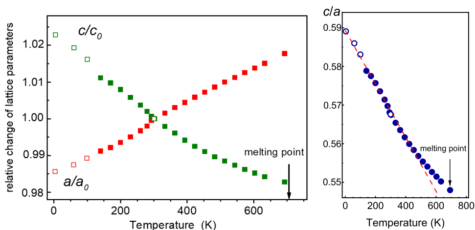
Figure 1. Relative changes of the lattice parameters vs temperature for the ambient pressure \text{CuReO}_4 -AP polymorph (left). The values were normalized to the lattice parameters at room temperature. Right: temperature dependence of the c/a ratio for \text{CuReO}_4 -AP together with the linear extrapolation of the data (red dashed line). Empty symbols correspond to the neutron powder diffraction data.
