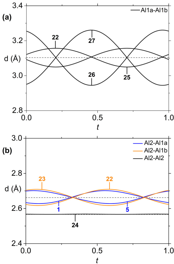
FIG. 7. t -Plots of interatomic distances (Å) in the CDW phase of \text{EuAl}_4 at 30 K. (a) d[\text{Al1a-Al1b}] with Al1a as central atom, and (b) d[\text{Al2-Al1a}] , d[\text{Al2-Al1b}] , and d[\text{Al2-Al2}] with Al2 as central atom. Basic structure distances are indicated by the dashed horizontal lines. t -Plots display variation in atomic parameters such as distance and position as a function of the phase t of the modulation wave [42]. Here, each value of t gives the distances from a central atom toward its neighboring atoms. The number on each curve is the number of the symmetry operator that is applied to the second atom of the bond pair. Symmetry operators are listed in Table S9 in the Supplemental Material [38].
