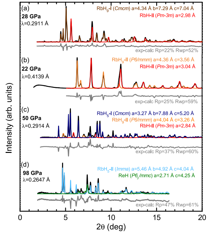
FIG. 1. Representative x-ray powder diffraction patterns and the results of the Rietveld refinements of (a) \text{RbH}_9\text{-I} at 28 GPa (brown), (b) \text{RbH}_9\text{-II} at 22 GPa (orange), (c) \text{RbH}_5\text{-I} at 50 GPa (dark blue), and (d) \text{RbH}_5\text{-II} at 98 GPa (light blue). The experimental data are shown by the black curves, and the refinement residuals are shown by the gray curves. The calculated contribution from \text{RbH}\text{-II} is shown in red, while \text{ReH} (from the gasket) is in green.
