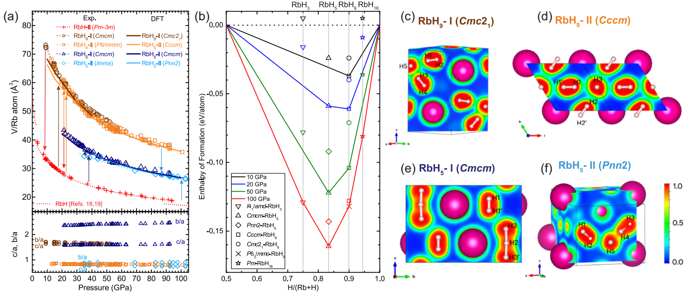
FIG. 2. (a) Volume as a function of pressure for the observed rubidium hydrides (top) and their b/a and c/a ratios (bottom). The dotted red curve shows the literature V(P) data for RbH [18,19], dashed curves indicate the Birch-Murnaghan fits with parameters listed in Table SMIII in Supplemental Material [25], and solid curves show the DFT predictions. Vertical arrows show minimal pressures at which the phase transitions were observed upon compression after heating and maximal pressures at which they were observed upon decompression. (b) Formation enthalpies ( \Delta H_F ) predicted by DFT for rubidium polyhydride phases (represented as different symbols) with respect to RbH + H_2 at 10 GPa (black), 20 GPa (blue), 50 GPa (green), and 100 GPa (red). Solid lines illustrate the convex hull. Calculated ELF plots for (c) Cmc2_1 - RbH_9 at 20 GPa, (d) Cccm - RbH_9 at 50 GPa, (e) Cmc2_1 - RbH_5 at 50 GPa, (f) Pnn2 - RbH_5 at 50 GPa. Cmc2_1 - RbH_5 possesses a linear symmetric H_3^- anion represented by atoms denoted H2, H3, and H3'. Pnn2 - RbH_5 possesses an asymmetric H_3^- anion comprised of atoms denoted H3, H4, and H5.
