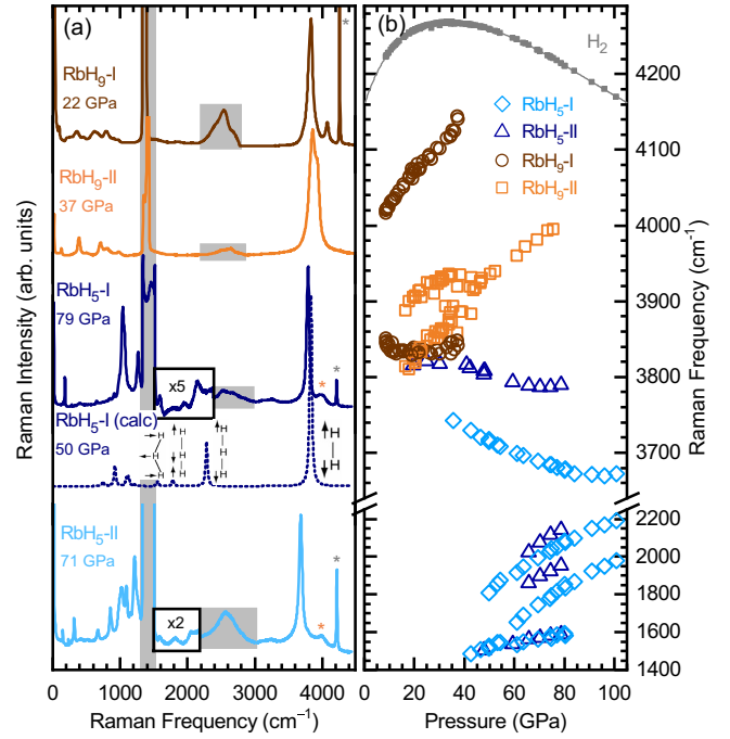
FIG. 3. (a) Representative Raman spectra of \text{RbH}_9\text{-I} (brown) at 22 GPa, \text{RbH}_9\text{-II} at 37 GPa (orange), \text{RbH}_5\text{-I} at 79 GPa (dark blue), and \text{RbH}_5\text{-II} at 71 GPa (light blue). The calculated Raman spectrum of Cmcm\text{-RbH}_5 at 50 GPa is shown as a dashed dark blue line, while the calculated Raman spectra of the other phases can be found in Fig. SM12 [25]. Raman excitations from the diamond anvils are highlighted by the gray shaded areas, gray asterisks indicate the vibron from the excess \text{H}_2 medium, and the orange asterisk indicates trace \text{RbH}_9\text{-II} . (b) Raman shift as a function of pressure of the vibrons attributed to quasimolecular hydrogen and \text{H}_3^- units within the rubidium lattices. The gray symbols correspond to the vibron frequency of the surrounding \text{H}_2 medium, while the gray line is the frequency of pure \text{H}_2 from prior studies [24]. The pressure dependence of the low frequency modes are given in Fig. SM3 [25].
