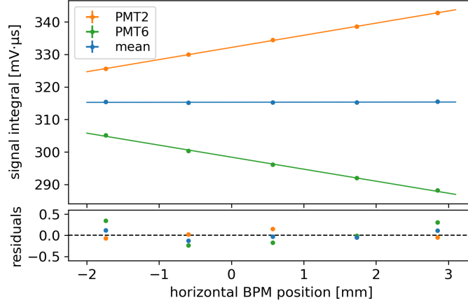
Figure 5: Signal integral of PMT2 (orange), PMT6 (green), and the mean of the two (blue) as a function of the horizontal position measured by the last BPM before the dump along with a linear fit. The residuals are shown below, representing the difference between the observed data and the fitted values.
