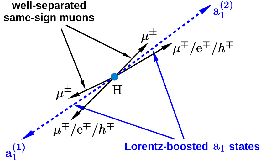
Figure 1: Illustration of the signal topology. The Higgs boson decays into two a_1 bosons, one of which further decays into a pair of tau leptons, and the other into a pair of muons or tau leptons. In the case of a_1 \rightarrow \tau\tau decays, one tau lepton is required to decay to a muon, and the other to a single charged particle—either an electron, a muon, or a charged hadron ( h ). The targeted final state consists of one muon and one oppositely charged track arising from each a_1 boson decay.
