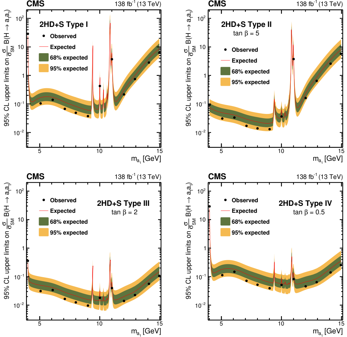
Figure 10: The observed (points) and expected (red line) 95% CL upper limits on \sigma(\text{pp} \rightarrow \text{H} + \text{X})\mathcal{B}(\text{H} \rightarrow a_1 a_1) , relative to \sigma_{\text{SM}} , as a function of m_{a_1} for different 2HD+S models at benchmark \tan \beta values: Type I ( \tan \beta independent; upper left), Type II ( \tan \beta = 5 ; upper right), Type III ( \tan \beta = 2 ; lower left), and Type IV ( \tan \beta = 0.5 ; lower right).
