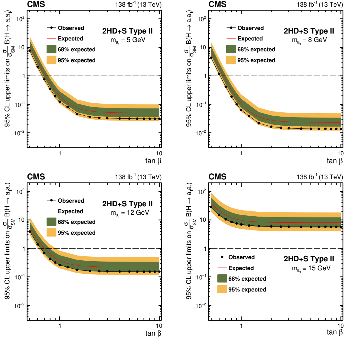
Figure 11: The observed (points) and expected (red line) 95% CL upper limits on \sigma(pp \rightarrow H + X) \mathcal{B}(H \rightarrow a_1 a_1) , relative to \sigma_{SM} , as a function of \tan \beta for the Type II 2HD+S model with m_{a_1} = 5 GeV (upper left), m_{a_1} = 8 GeV (upper right), m_{a_1} = 12 GeV (lower left), and m_{a_1} = 15 GeV (lower right).
