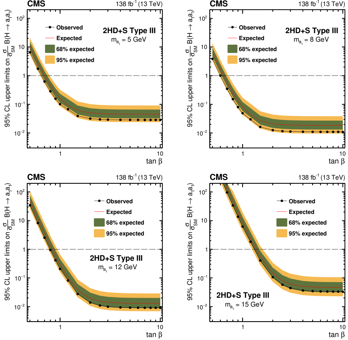
Figure 12: The observed (points) and expected (red line) 95% CL upper limits on \sigma(pp \rightarrow H + X) \mathcal{B}(H \rightarrow a_1 a_1) , relative to \sigma_{SM} , as a function of \tan \beta for the Type III 2HD+S model with m_{a_1} = 5 GeV (upper left), m_{a_1} = 8 GeV (upper right), m_{a_1} = 12 GeV (lower left), and m_{a_1} = 15 GeV (lower right).
