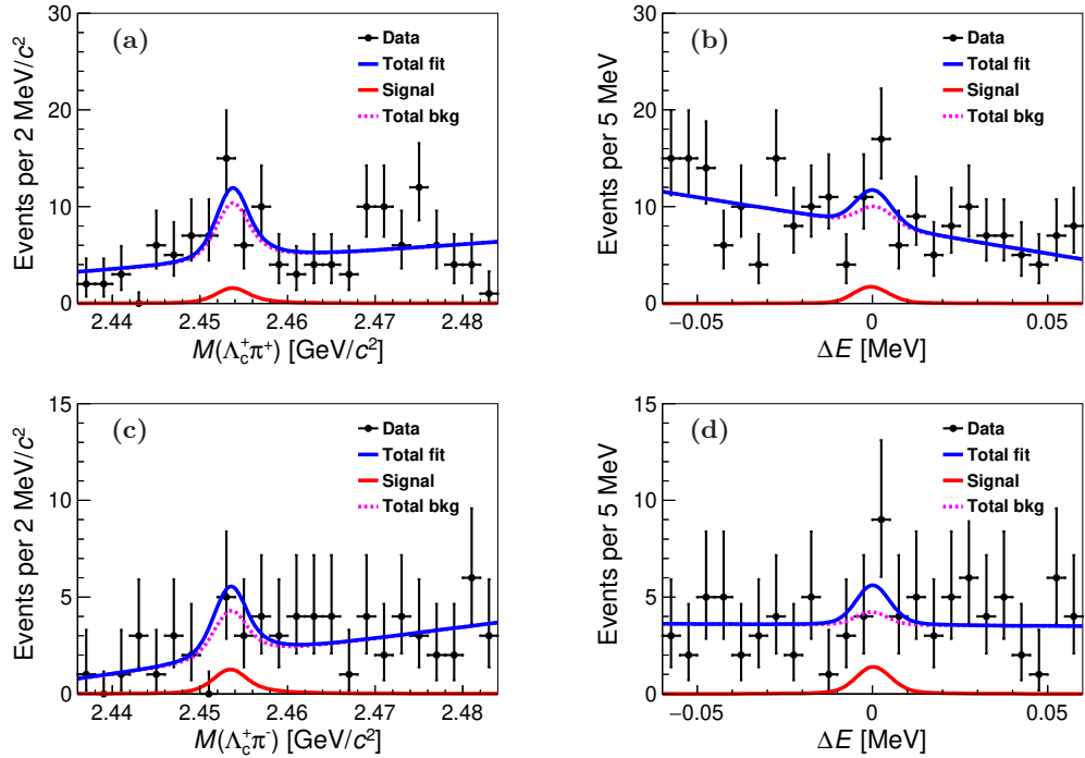
FIG. 3: Distributions of (a, c) M(\Lambda_c^+ \pi^\pm) and (b, d) \Delta E for the reconstructed (top) B^+ \rightarrow \Sigma_c(2455)^{++} \Xi_c^{--} and (bottom) B^0 \rightarrow \Sigma_c(2455)^0 \Xi_c^{0-} candidates, using events from the sideband regions of M(\Xi_c^{0-}) in the combined Belle and Belle II data sets. All components are indicated in the legends.
