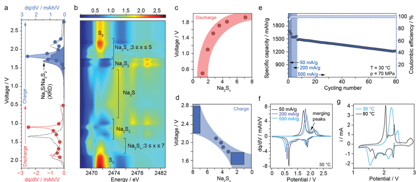
Figure 4. | Ex situ soft XAS and electrochemical analysis (a) dQ/dV plot of solid-state Na–S battery employing \text{Na}_3\text{PS}_4 (80 °C; dashed line) or \text{Na}_4(\text{B}_{10}\text{H}_{10})(\text{B}_{12}\text{H}_{12}) (30 °C; solid line). Red and blue dots indicate the voltage where individual cells had been stopped for XAS studies. Blue highlighted peaks indicate the merging of two contributions due to changing kinetics. (b) Contour plot of the ex-situ XAS of the solid-state Na–S battery, showing the discharge cycle and charging cycle. Highlighted regions showing the corresponding XAS spectra of the different polysulfides, grouping the high-ordered \text{Na}_2\text{S}_x , x = 3–7 . (c) Formation plot of the different polysulfides during discharge, and in (d) during charge, showing the formation voltage vs \text{Na}_2\text{S}_x sodiation. (e) Cycling performance of the solid-state Na–S battery employing \text{Na}_4(\text{B}_{10}\text{H}_{10})(\text{B}_{12}\text{H}_{12}) at a rate of 500 mA/g at 30 °C, with a few formation cycles at rates of 50 and 100 mA/g to ensure proper formation of the battery's internal structure and chemistry. (f) Selected dQ/dV plot based on (e) for 50, 200, and 500 mA/g. The arrow indicates peak merging with higher current densities. (g) Cyclic voltammogram of solid-state Na–S battery employing \text{Na}_4(\text{B}_{10}\text{H}_{10})(\text{B}_{12}\text{H}_{12}) at 30 and 80 °C, scanned at 25 \mu\text{V/s} and 10 mV/s, respectively.
