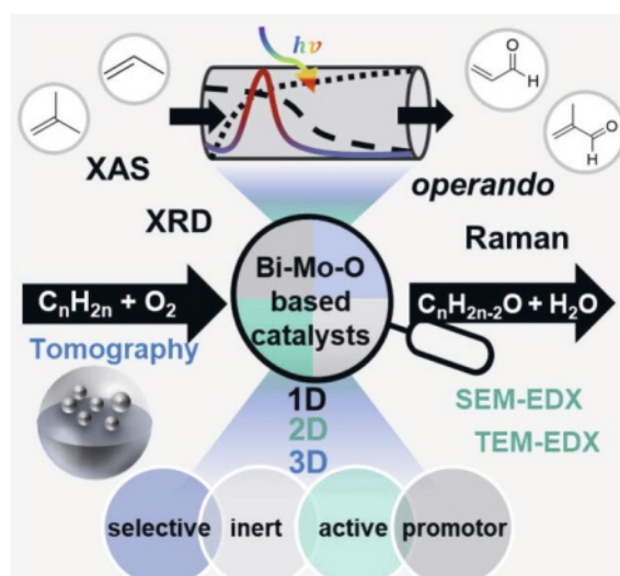
Fig. 5. Toolbox of advanced characterization techniques for deriving structural information of Bi-Mo-O-based catalysts for selective oxidation of olefins under operando conditions. Reproduced with permission from ref. [46].
