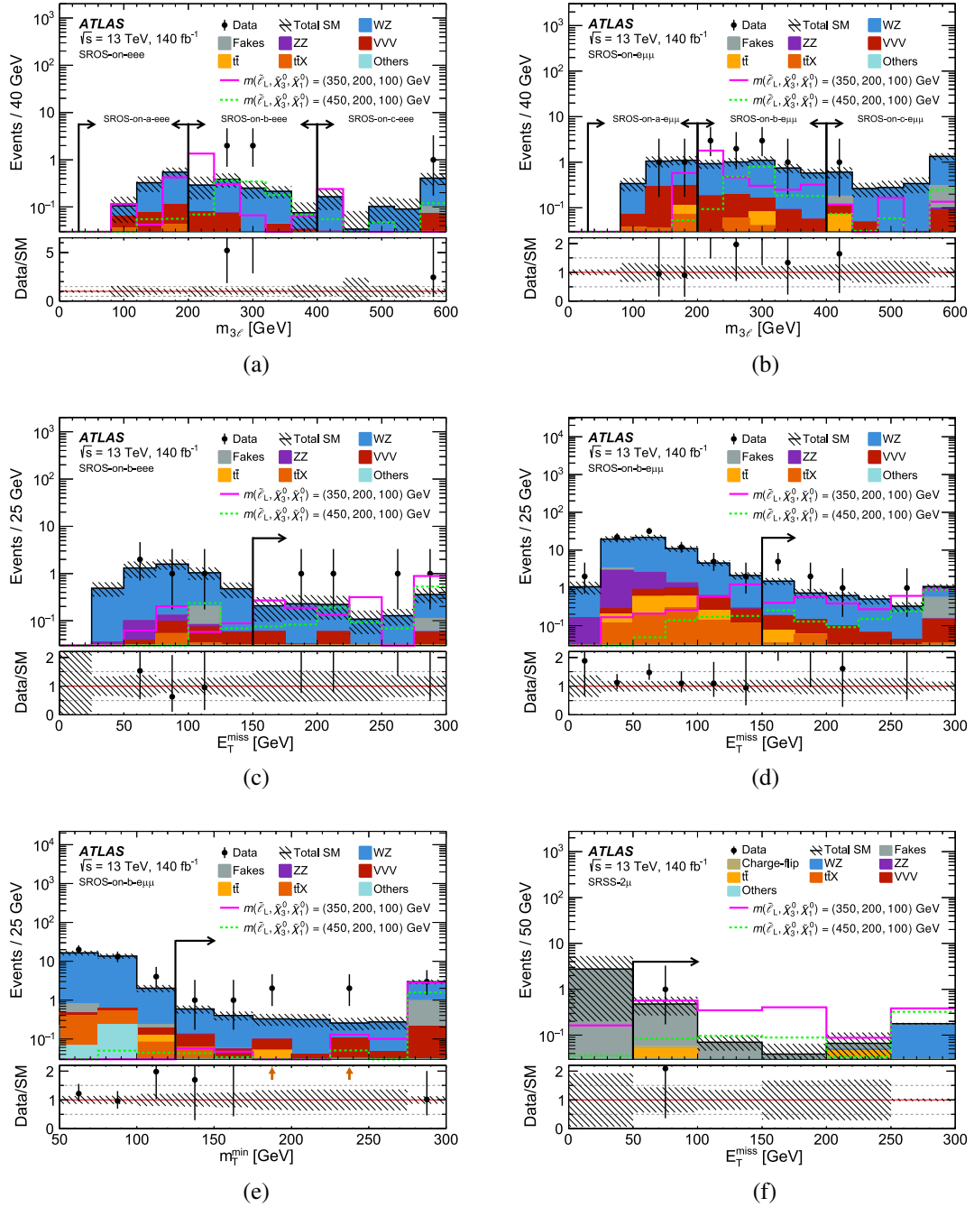
FIG. 14. Distributions of m_{3\ell} in (a) SROS-on- eee and (b) SROS-on- e\mu\mu , of E_T^{\text{miss}} in (c) SROS-on-b- eee and (d) SROS-on-b- e\mu\mu , of (e) m_T^{\text{min}} in SROS-on-b- e\mu\mu , and of (f) E_T^{\text{miss}} in SRSS- 2\mu . The SR selections are applied for each distribution, except for the variable shown, for which the selection is indicated by a black arrow. The last bin includes the overflow. The Others category contains the production of Higgs boson, 3-top, 4-top, and single-top processes. Distributions for SBH signals are overlaid. The bottom panels show the ratio of the observed data to the predicted total background yields. Ratio values outside the graph range are indicated by brown arrows. The hatched band includes all statistical and systematic uncertainties.
