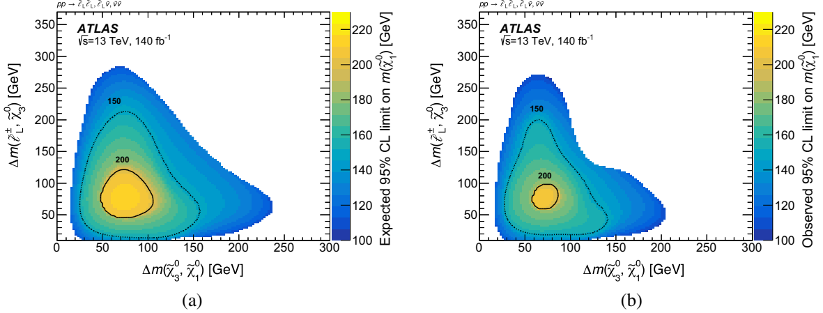
FIG. 17. The (a) expected and (b) observed lower limit on the \tilde{\chi}_1^0 mass at 95% CL. The limits are shown onto the \Delta m(\tilde{e}_L, \tilde{\chi}_3^0) vs \Delta m(\tilde{\chi}_3^0, \tilde{\chi}_1^0) plane. The dotted (solid) contour line indicate 150 (200) GeV limit of \tilde{\chi}_1^0 mass. In the white region, the lower limit on the \tilde{\chi}_1^0 mass is below 100 GeV.
