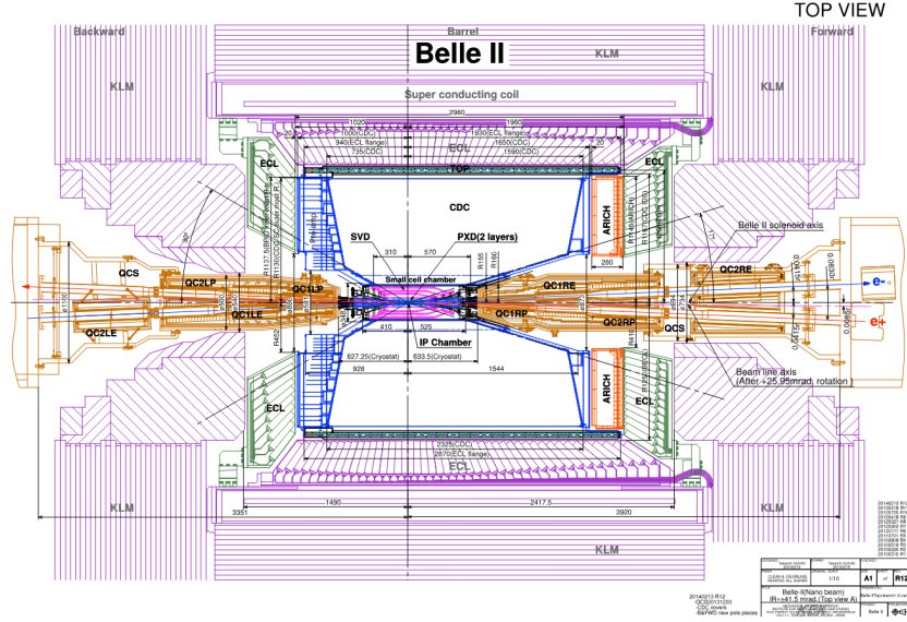
Figure 3.5: An overhead view of a slice of the Belle II detector, illustrating the interaction region and the different sub-detector systems. The drawing is taken from “The Belle II Physics Book” [15]
