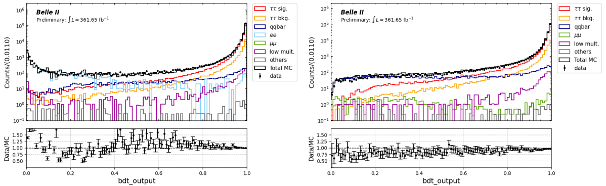
Figure 5.18: First step BDT output distributions for electron (left) and muon (right) channel, in logarithmic y-axis scales.
