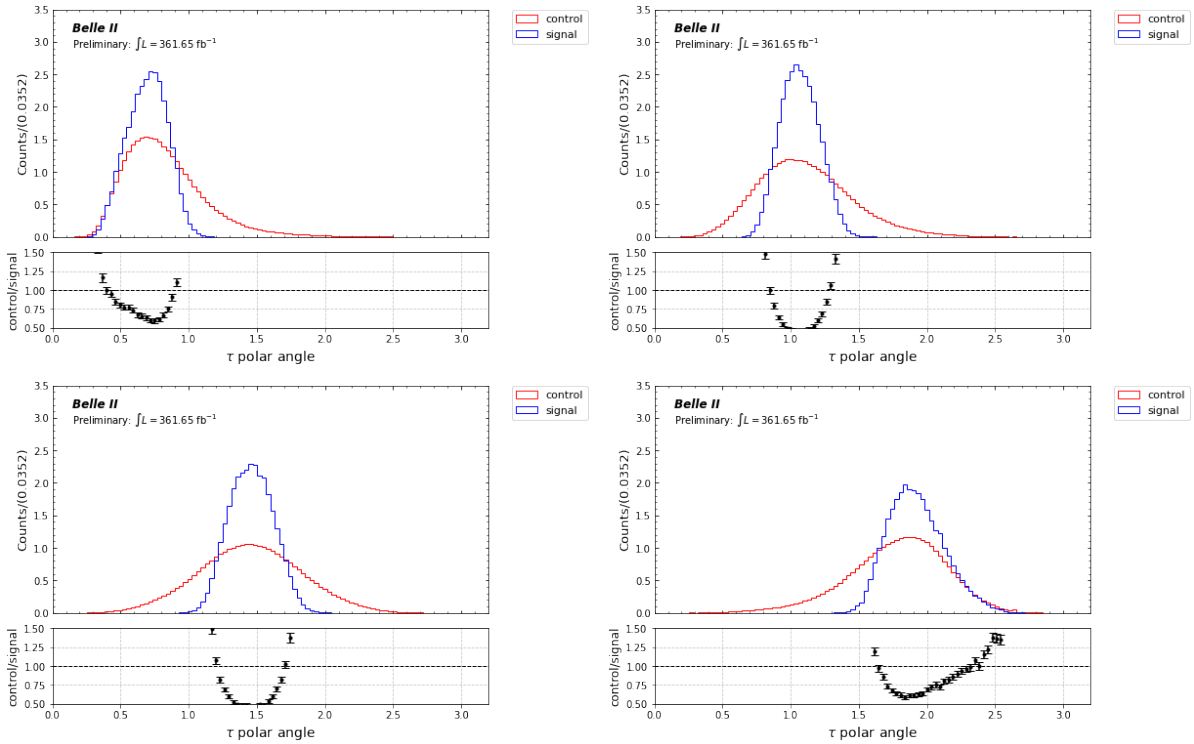
Figure 7.4: \tau polar angle (in CMS) distribution for each K_S^0 polar angle bin. The control sample is shown in red and the signal sample in blue, normalized to unit area.
