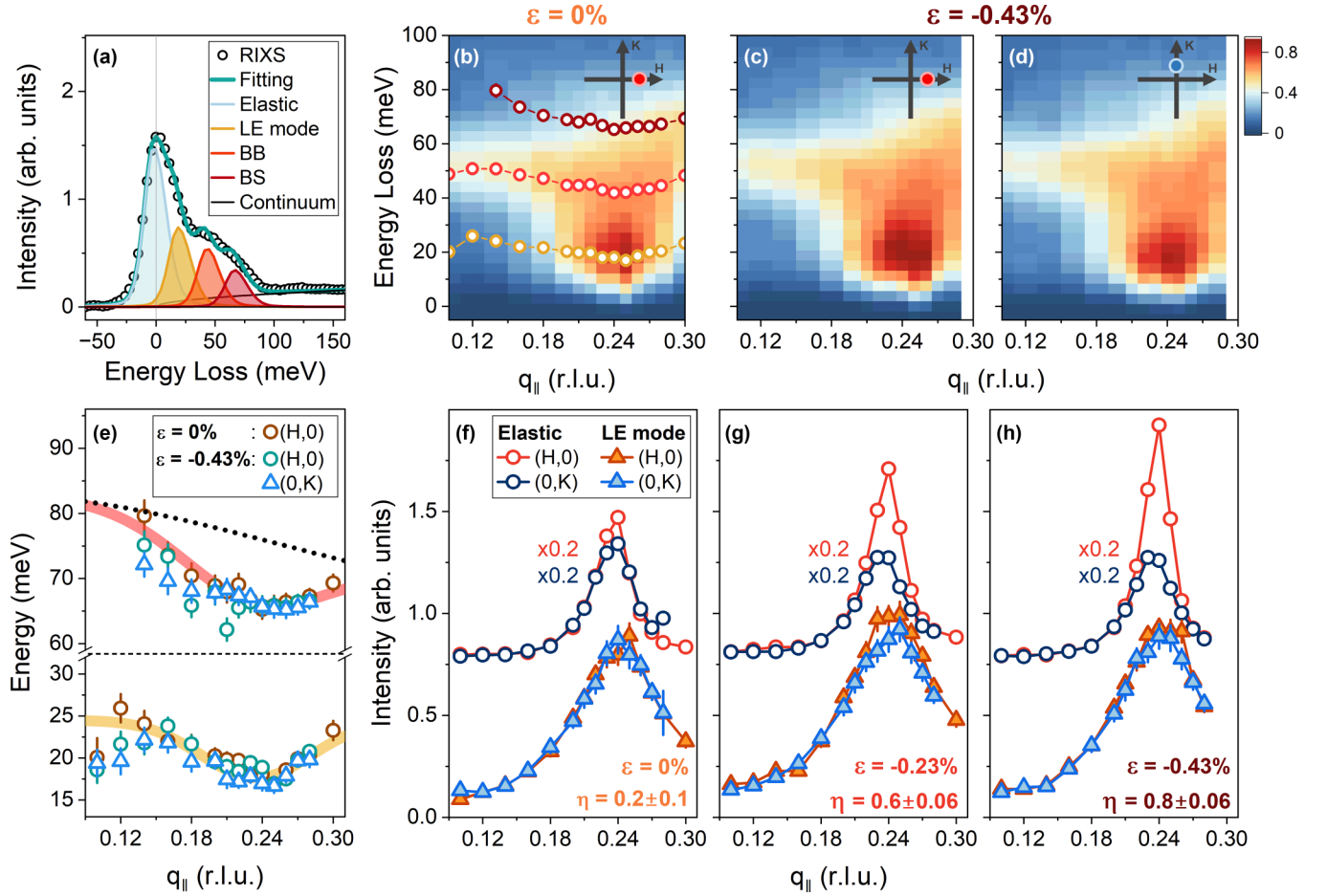
FIG. 2. Oxygen- K edge resonant x-ray scattering. (a) Example of a fitted spectrum at Q=(0.26,0) . (b)–(d) RIXS spectra as a function of momentum q_{||} after subtraction of the elastic signal. Applied strain values and directions are indicated above the panels and in the insets, respectively. (e) Energy of the bond-stretching mode and of the low-energy mode as a function of momentum for two different values of applied strain, for both H (circles) and K (triangles) directions. The black dotted line is a cosine function, while the red and yellow solid lines are guides to the eye. (f)–(h) Intensity of elastic peak (empty circles) and low-energy mode (filled triangles) for both (H, 0) (red and orange symbols) and (0, K) (blue and light-blue symbols) directions, for increasing strain application.
