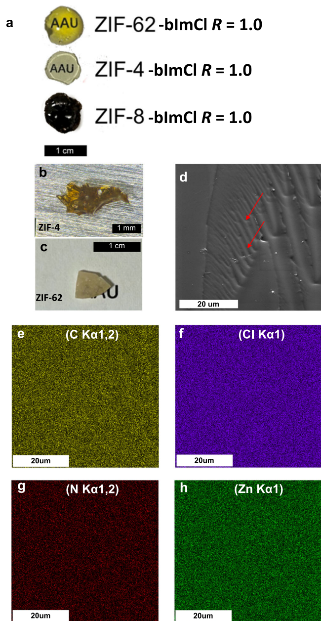
Fig. 2 | Photographs, SEM images, and compositional mapping of \text{H}_2\text{blmCl} modified ZIF-derived glasses. a Photographs of blmCl-modified ZIF-4, ZIF-8, and ZIF-62 ( R = 1.0 ) glasses after melt-quenching. Clear transparency is observed for the ZIF-4-blmCl and ZIF-62-blmCl samples. b, c Photographs of unmodified: b ZIF-4 and c , ZIF-62 glasses. Note the scale differences in ( a–c ). d SEM image of a ZIF-4-blmCl ( R = 1.0 ) glass, showing smooth viscous flow and fracture lines, suggesting the existence of a liquid-like state during forming (red arrows). EDX measurements of ZIF-4-blmCl R = 1.0 glass for e C, f Cl, g N, and h Zn elements.
