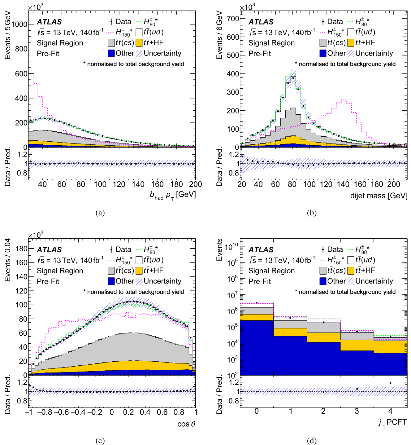
Fig. 4 Distributions of selected BDT input variables. The variables are defined in Table 2. The processes t\bar{t}(\text{allHad}) , t\bar{t}W , Single top, t\bar{t}H , Other top, W + \text{jets} , Z + \text{jets} , VV listed in Table 1 are combined with the multijet background in the “Other” category. The uncertainty band
