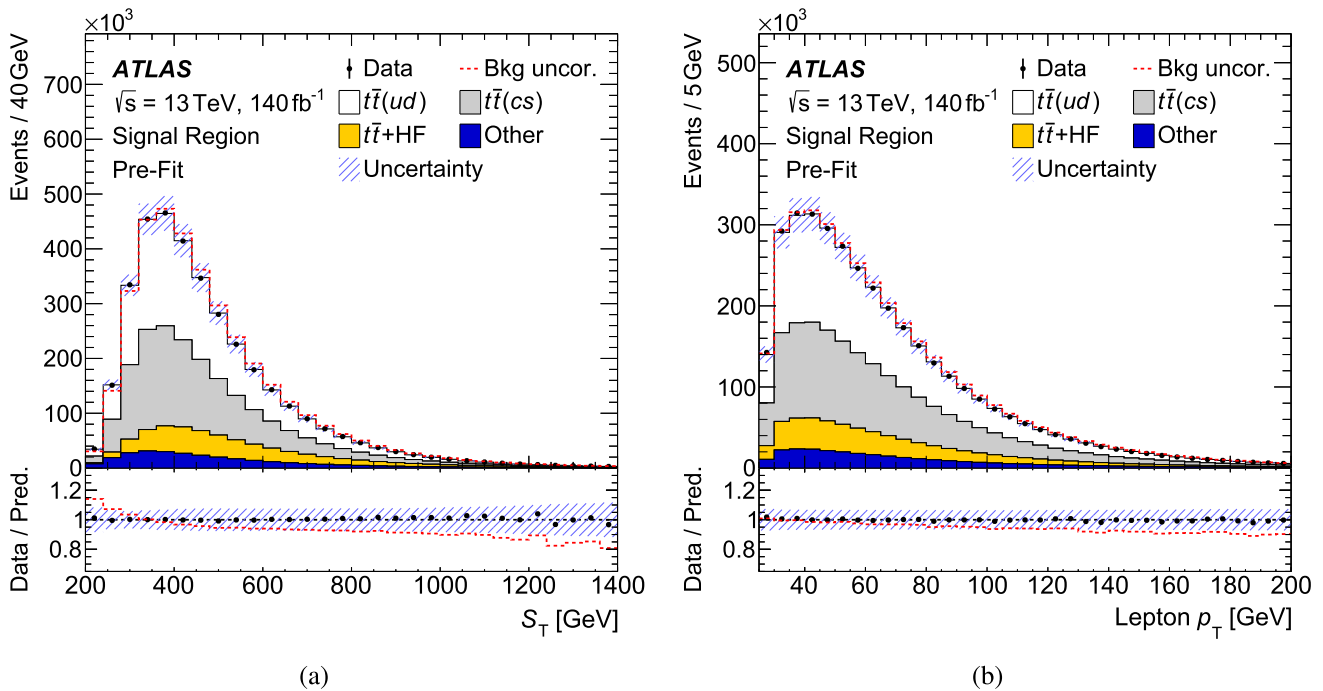
Fig. 2 Distribution of a S_T and b lepton p_T after applying the t\bar{t} correction. The processes t\bar{t}(\text{allHad}) , tW , Single top, t\bar{t}H , Other top, W + \text{jets} , Z + \text{jets} , and VV listed in Table 1 are combined with the multijet background in the “Other” category. The uncertainty band represents the
