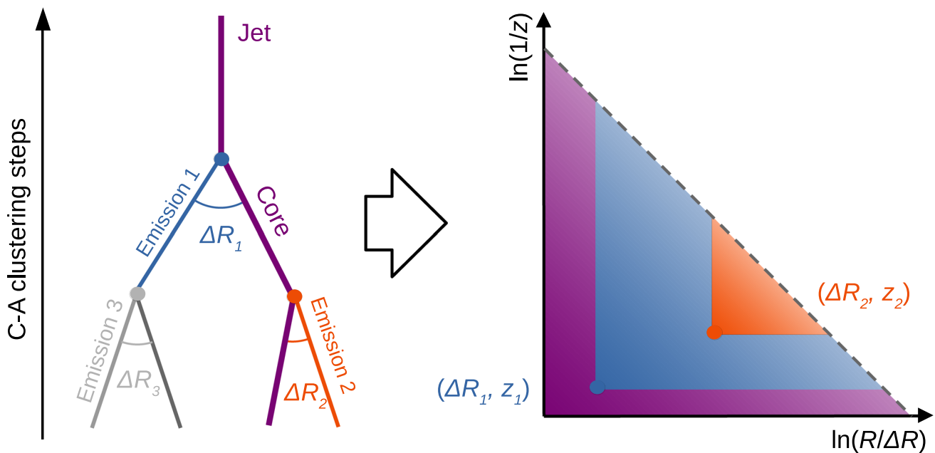
Fig. 1 Illustration showing the process by which the LJP is constructed. The CA algorithm clusters pairs of proto-jets according to angular separation \Delta R . At each step, the higher- p_T proto-jet is considered to be the core and the lower- p_T one the emission. The variables \ln(R/\Delta R) and \ln(1/z) are plotted on the LJP for each emission origi-
