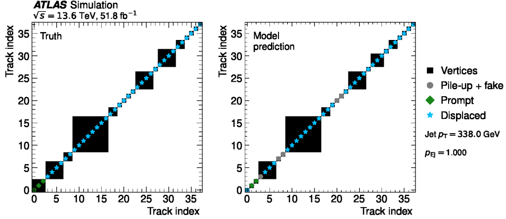
Figure 5: Example of the auxiliary task performance on a single jet with p_{\text{EJ}} = 1.000 from a sample of simulated signal events with m_{Z'} = 1500 GeV, m_{\pi_D} = 10 GeV, and c\tau_{\pi_D} = 50 mm. The reconstructed tracks in the jet are shown along the diagonal and are displayed using different markers based on their origin, with displaced tracks shown as stars, prompt tracks shown as diamonds, and both pile-up and fake tracks shown as circles. Groups of tracks that form a common vertex are shown as filled squares. The left diagram shows the true track and vertex labels, and the right diagram shows the model predictions. Track indices are ordered such that tracks originating from the same truth vertex appear consecutively.
