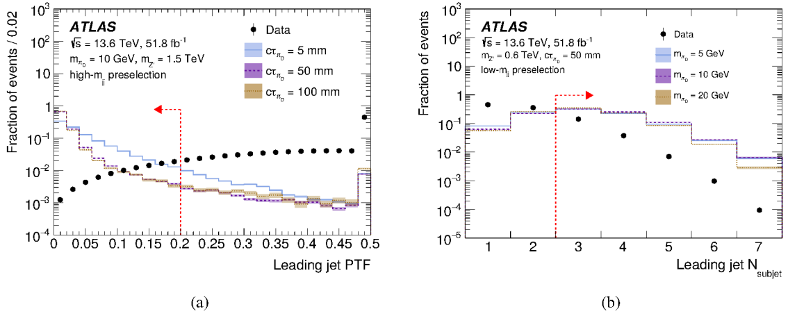
Figure 4: Normalised distributions of (a) the leading jet PTF in the high- m_{jj} preselection and (b) the leading jet number of subjets in the low- m_{jj} preselection in signal events (lines) and data (circles). The selection applied to the observable to define the signal region is indicated by a dashed arrow. The rightmost bins include contributions from overflow events.
