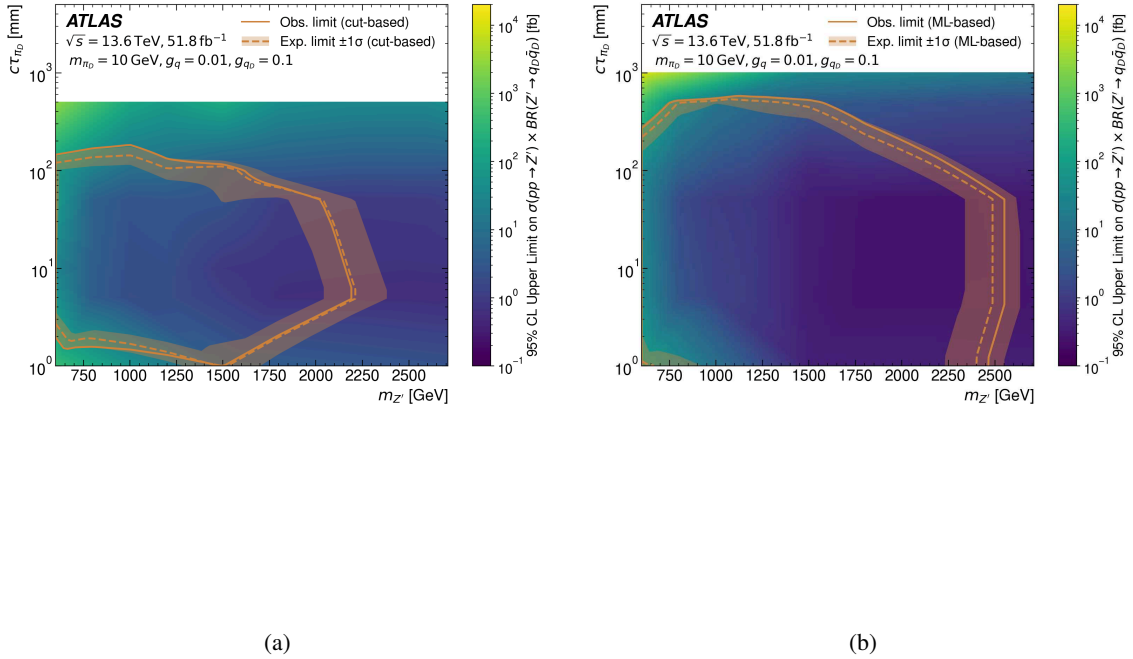
Figure 10: The 95% CL exclusion limits on \sigma(pp \rightarrow Z') \times \text{Br}(Z' \rightarrow qD\bar{q}_D) as a function of m_{Z'} and c\tau_{\pi_D} for (a) the cut-based analysis and (b) the ML-based analysis. The excluded region computed from the observed limits for g_q = 0.01 and g_{qD} = 0.1 is shown as a solid line.
