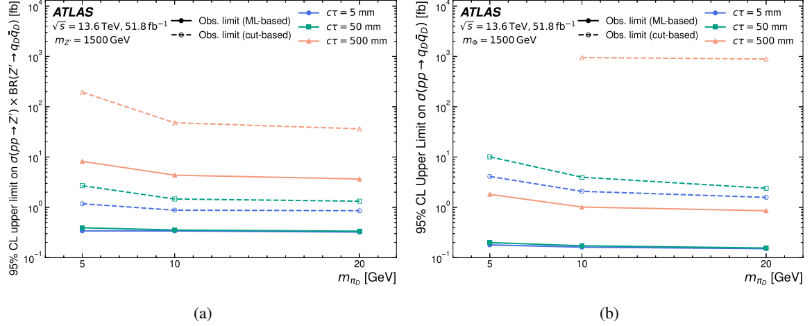
Figure 12: The 95% CL exclusion limits on (a) \sigma(pp \rightarrow Z') \times \text{Br}(Z' \rightarrow q_D \bar{q}_D) and (b) \sigma(pp \rightarrow q_D \bar{q}_D) for m_{Z',\Phi} = 1500 GeV for the cut-based (hollow markers and dashed lines) and ML-based (filled markers and solid lines) strategies. The limits are shown for c\tau_{\pi_D} = 5 mm (circles), 50 mm (squares) and 500 mm (triangles).
