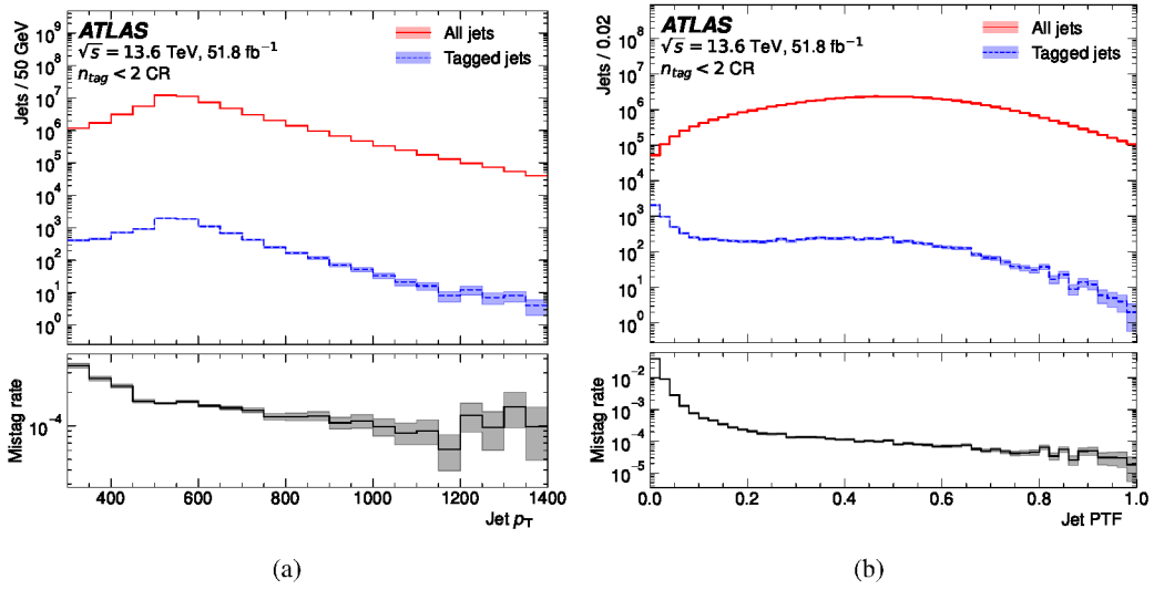
Figure 9: Distributions of (a) p_T and (b) PTF for all jets (solid lines) and jets with a classification score greater than 0.98 (dashed lines) in the high- m_{jj} selection for data events with n_{tag} < 2 . The bottom panel shows the mistag rate as a function of each observable.
