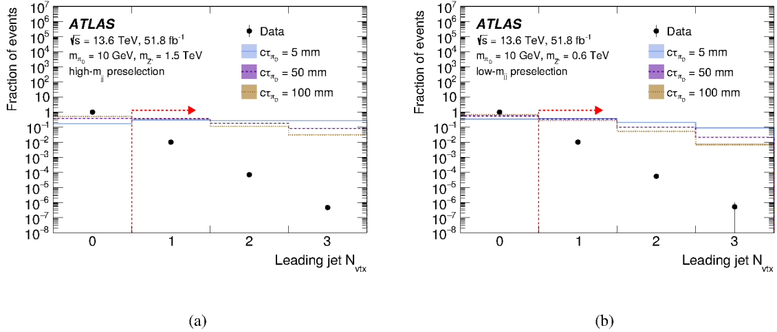
Figure 3: Normalised distributions of N_{\text{vtx}} for the leading jet in (a) the high- m_{jj} preselection and (b) the low- m_{jj} preselection for signal events (lines) and data (circles). The selection placed on the observable in the analysis is indicated with a dashed arrow. The rightmost bins include contributions from overflow events.
