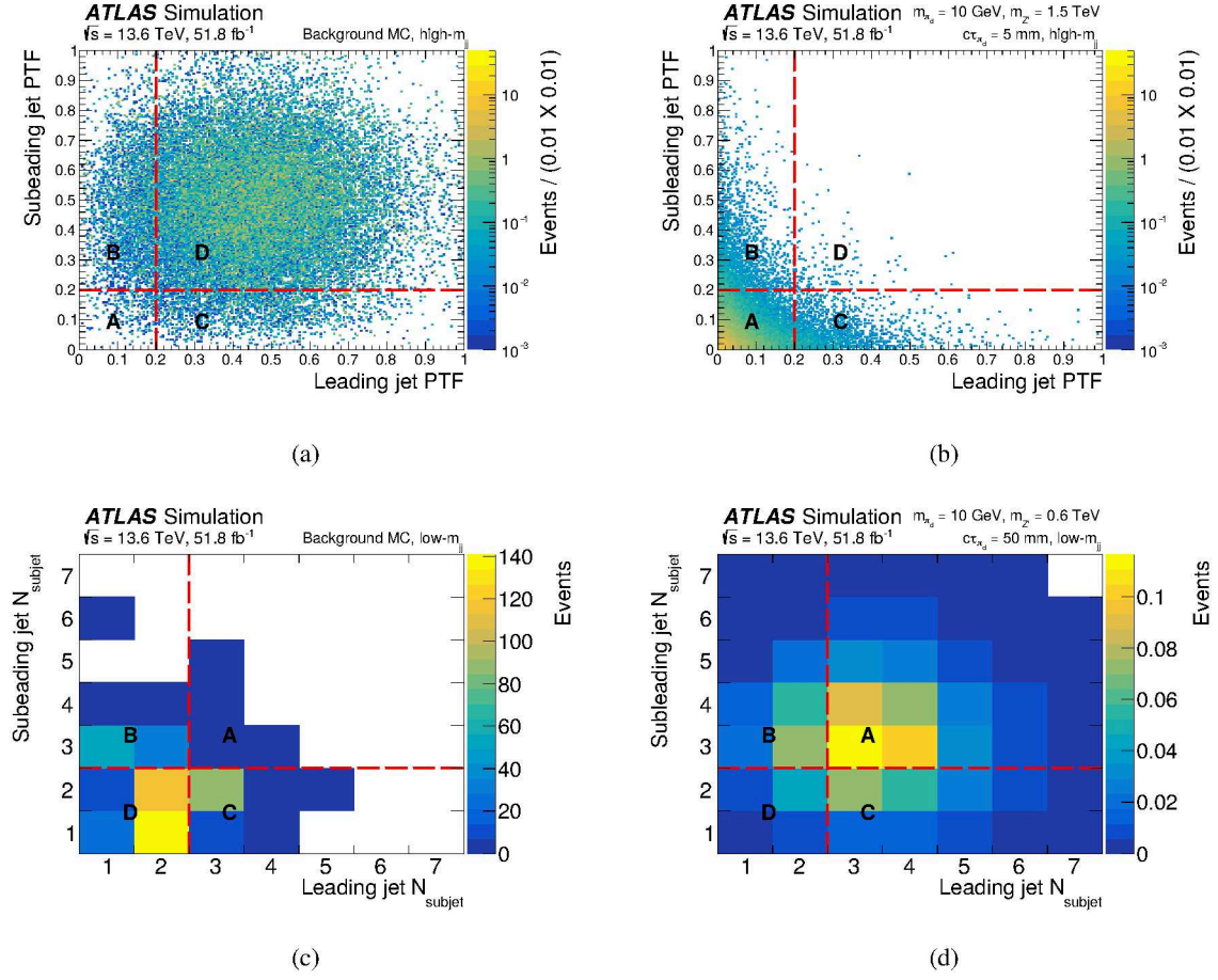
Figure 7: The distributions of (a,c) simulated background events (b,d) and signal events in the (a,b) high- m_{jj} region and (c,d) low- m_{jj} region (bottom). The parameters of the simulated signal shown in (b) corresponds to m_{Z'} = 1.5 TeV, m_{\pi_D} = 10 GeV, c\tau_{\pi_D} = 5 mm and the signal shown in (d) corresponds to m_{Z'} = 0.6 TeV, m_{\pi_D} = 10 GeV and c\tau_{\pi_D} = 50 mm.
