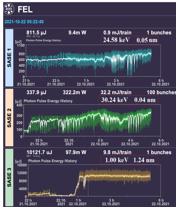
Figure 6. First test run of the EuXFEL delivering hard X-rays of about 0.8 mJ and 0.3 mJ at photon energies of 24 keV and 30 keV for SASE beamlines 1 and 2, respectively, with a simultaneous SASE pulse delivery of about 10 mJ at 1 keV for the SASE beamline 3.
