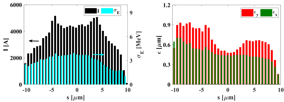
Figure 3. Bunch qualities in front of the undulator beamline SASE1. Left: peak current (left axis) and slice energy spread (right axis); Right: slice horizontal (green) and vertical (red) emittance.
