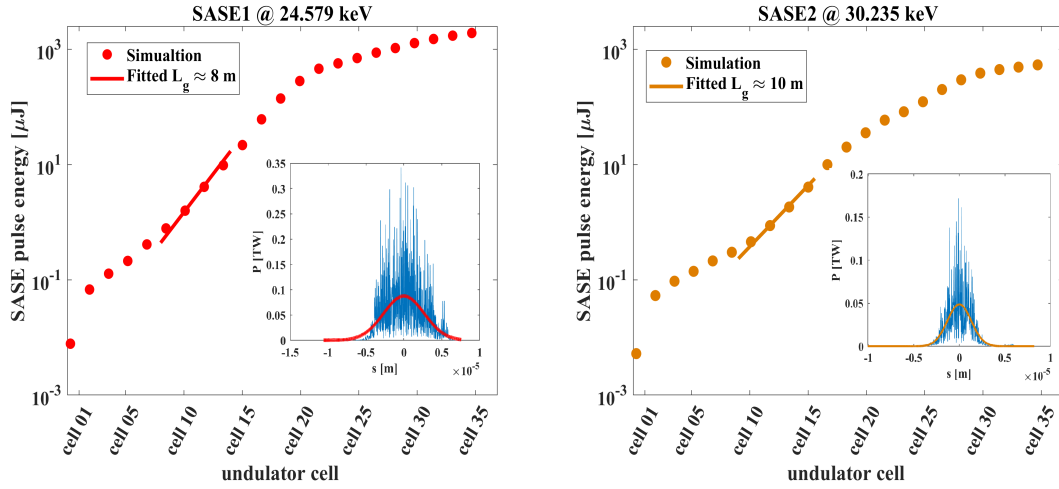
Figure 4. Simulated SASE intensities at 24.58 keV (left) and 30.24 keV (right) for beamlines SASE1 and SASE2, respectively.
