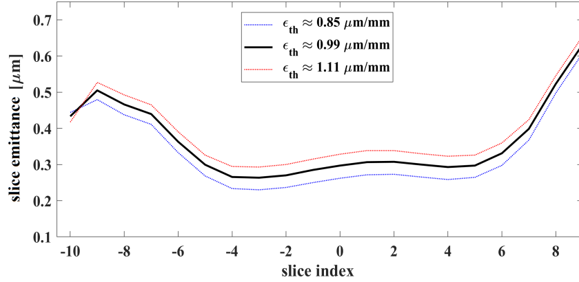
Figure 2. Optimized slice emittance at the injector exit considering different thermal emittance values of the cesium-telluride cathodes as tested at PITZ [19].
