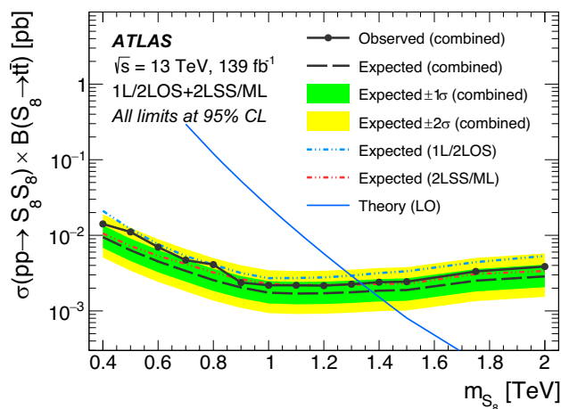
Fig. 12 Expected and observed 95% CL upper limits on the S_8S_8 \rightarrow t\bar{t}t\bar{t} production cross-section as a function of m_{S_8} , obtained from the combination of the 1L/2LOS and 2LSS/ML final states. The expected limits from the individual 1L/2LOS and 2LSS/ML analyses are also shown. The predicted production cross-section from Ref. [34] is shown with the solid blue curve
