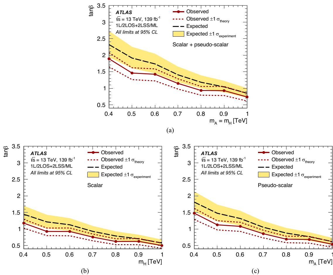
Fig. 11 Expected (black dashed line) and observed (red solid line) 95% CL limits on \tan\beta as a function of the m_{H/A} mass obtained using the combination of 1L/2LOS and 2LSS/ML final states, assuming type-II 2HDM in the alignment limit. Values of \tan\beta below the observed limit are excluded. The scenario where both the scalar H and pseudo-scalar A contribute with m_H = m_A is shown in a . The scenarios with the
