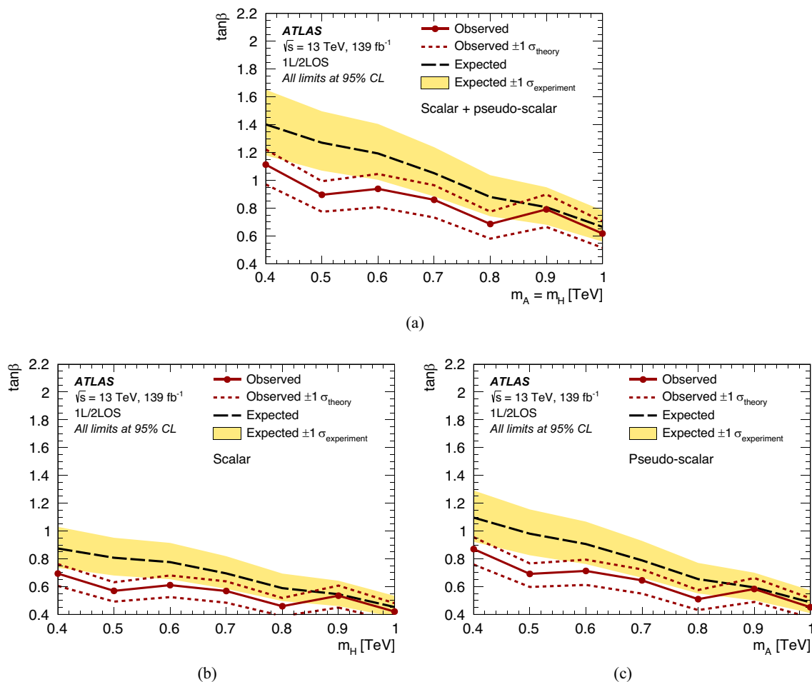
Fig. 9 Observed (red solid line) and expected (black dashed line) 95% CL lower limits on \tan \beta as a function of the m_{H/A} mass obtained using the 1L/2LOS final states, assuming a Type-II 2HDM in the alignment limit. Values of \tan \beta below the observed limit are excluded. The scenario where both the scalar H and pseudo-scalar A contribute with m_H = m_A is shown in a . The scenarios with the contribution from H
