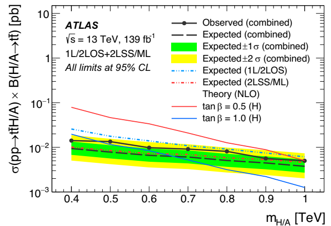
Fig. 10 Expected and observed 95% CL upper limits on the cross-section times branching ratio, \sigma(pp \rightarrow t\bar{t}H/A) \times B(H/A \rightarrow t\bar{t}) , as a function of m_{H/A} , obtained from the combination of the 1L/2LOS and 2LSS/ML final states. The green (yellow) band illustrates the \pm 1\sigma ( \pm 2\sigma ) interval around the expected limit from the combination. The expected limits from the individual 1L/2LOS and 2LSS/ML analyses are also shown. Theoretical predictions for two values of \tan\beta are shown for an H boson. The predicted values for A differ by less than 3% for all mass points for the two \tan\beta values shown
