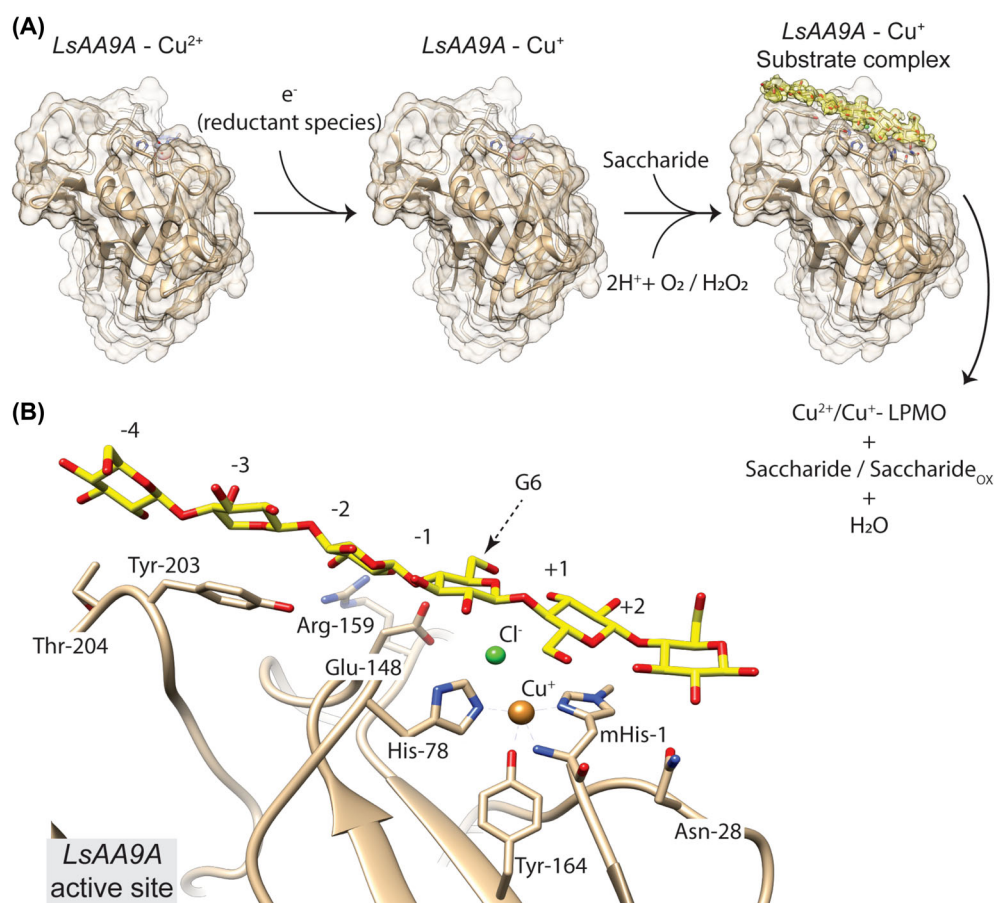
Fig. 1. Overall structure and reaction scheme of LsAA9A . (A) Overall structure of LsAA9A (PDB code 5ACG) (ribbon diagram) and reaction scheme for its peroxxygenase activity on cellooligosaccharides; (B) Close-up visualization of the LsAA9A \text{Cu}^+ (PDB code 5ACH) active site with bound cellohexaose (G6) moiety, with subsite numbering indicated. The N-terminal methylated histidine, histidine 78, and tyrosine 164 forming the active site are shown. The exogenous \text{Cl}^- ion, presumed to mimic the oxygen species during the LPMO saccharide cleavage, is shown. Figures were generated using UCSF ChimeraX [51].
