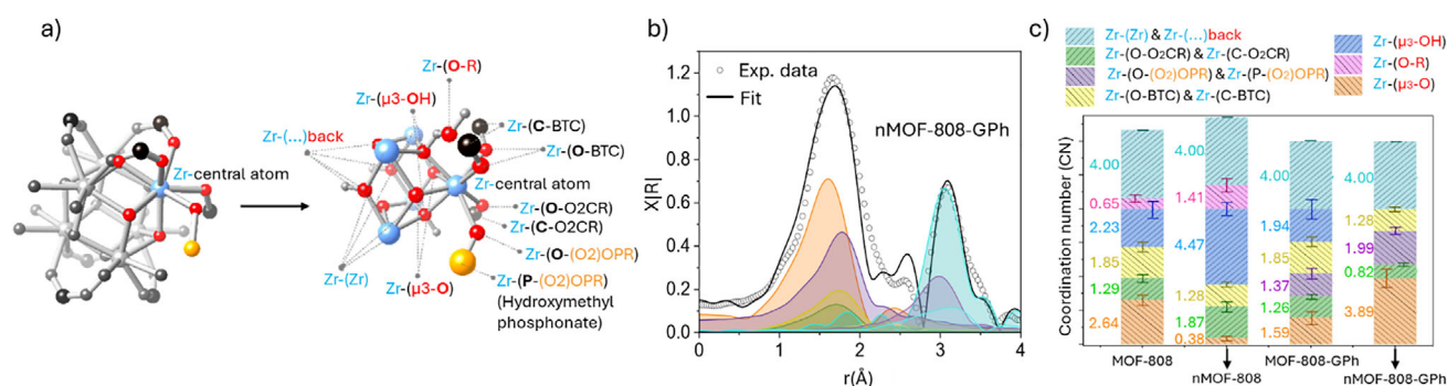
Figure 5. a) Description of scattering paths used in EXAFS refining. b) EXAFS fit of nMOF-808-GPh showing scattering paths contributions as described in a) (K weight 2, \Delta k = 3.0\text{--}11.3\text{ \AA}^{-1} ; \Delta R = 1.0\text{--}4.0\text{ \AA} ). c) Comparison of CN for each scattering path as described in a), for MOFs before and after reaction (the color code for legends of scattering paths is the same in b) and c).
