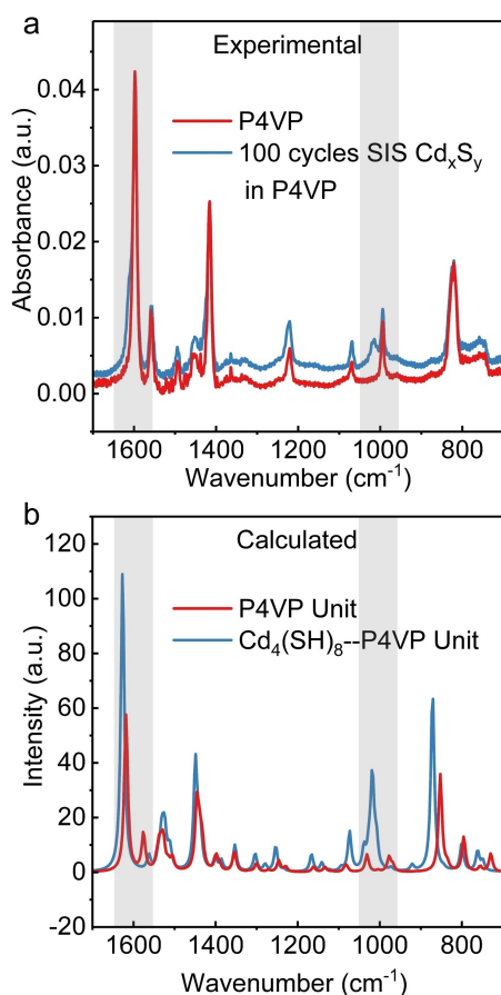
Figure 6. Experimental vs calculated FTIR spectra comparison before and after SIS processing at 80 °C in P4VP matrix. a) Experimental P4VP and 100 cycle SIS spectra b) DFT calculated P4VP unit and \text{Cd}_4(\text{SH})_8 P4VP one unit adduct at the B3LYP-D3/CEP-121G level of theory. The grey areas highlight infrared energies where significant intensity changes are simulated and observed.
