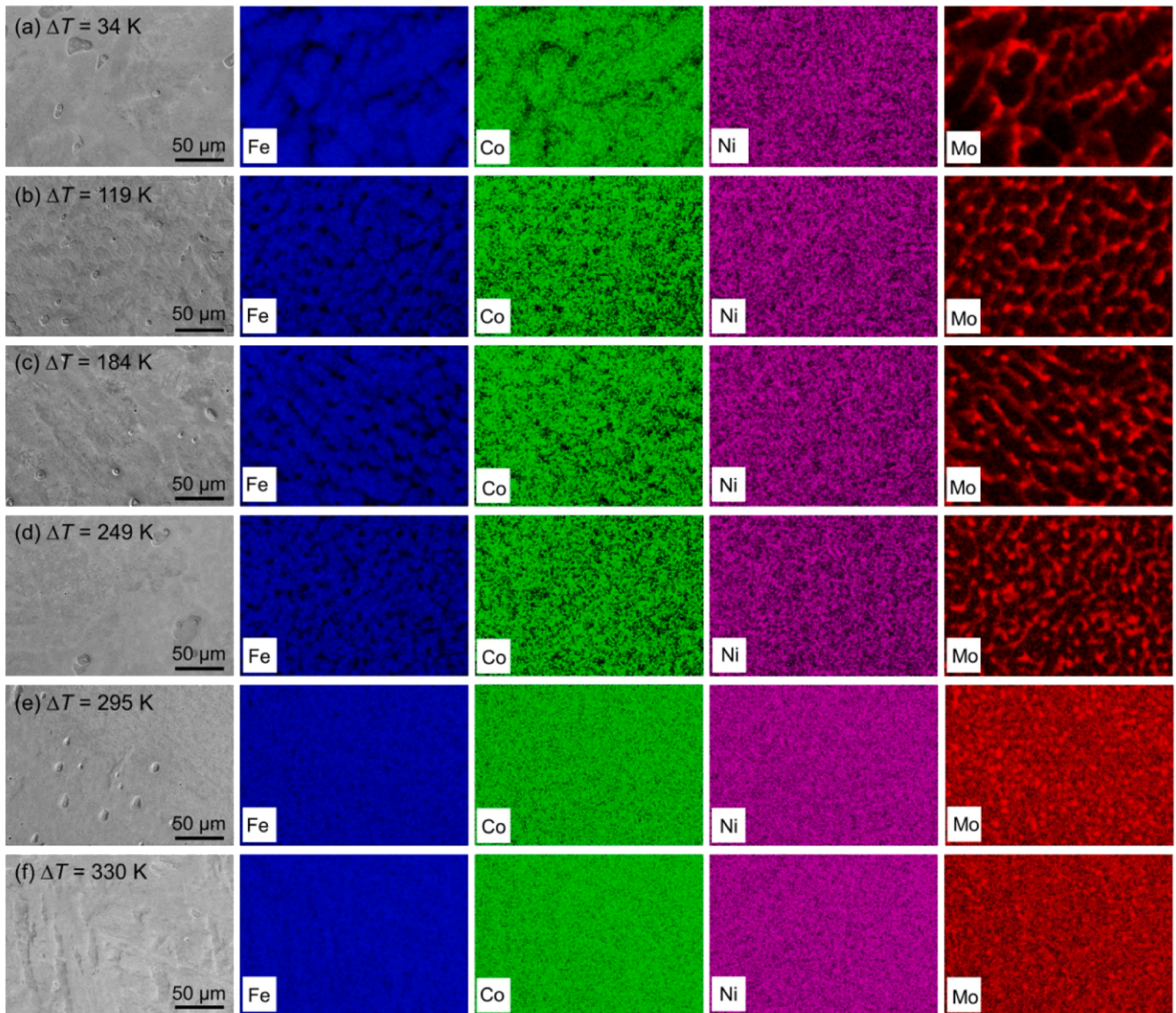
Fig. 11. SEM SEI overview images and EDS element distribution maps for \text{Fe}_{60}\text{Co}_{25}\text{Ni}_{10}\text{Mo}_5 samples solidified at different melt undercooling: (a) \Delta T = 34 K; (b) \Delta T = 119 K; (c) \Delta T = 184 K; (d) \Delta T = 249 K; (e) \Delta T = 295 K; (f) \Delta T = 330 K.
