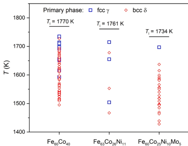
Fig. 5. Nucleation statistics for \delta and \gamma phases emerging as a primary crystalline phase in \text{Fe}_{60}\text{Co}_{40} [16], \text{Fe}_{63}\text{Co}_{26}\text{Ni}_{11} and \text{Fe}_{60}\text{Co}_{25}\text{Ni}_{10}\text{Mo}_5 undercooled melts.
