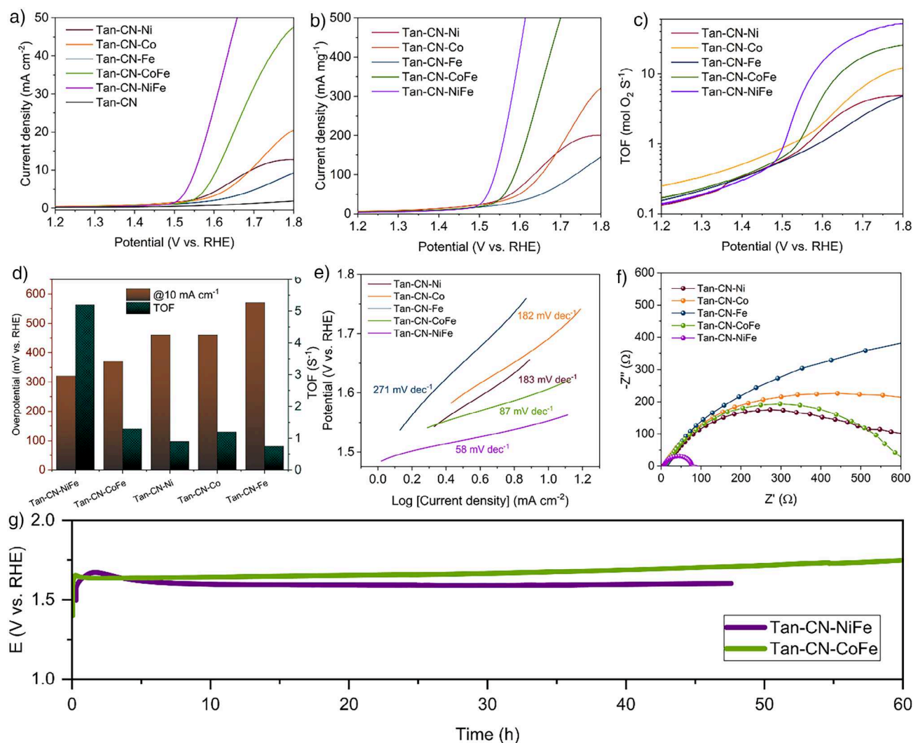
Figure 3. a) LSV curves with a scan rate of 10 \text{ mV s}^{-1} , b) corresponding mass activities, and c) TOF curves of the as-prepared catalysts. d) Overpotentials and TOFs at the current density of 10 \text{ mA cm}^{-2} . e) Tafel slopes. f) EIS curves at 1.5 \text{ V} versus RHE. g) Chronopotentiometry measurements of CoFe and NiFe SACs at 10 \text{ mA cm}^{-2} on carbon cloth.
