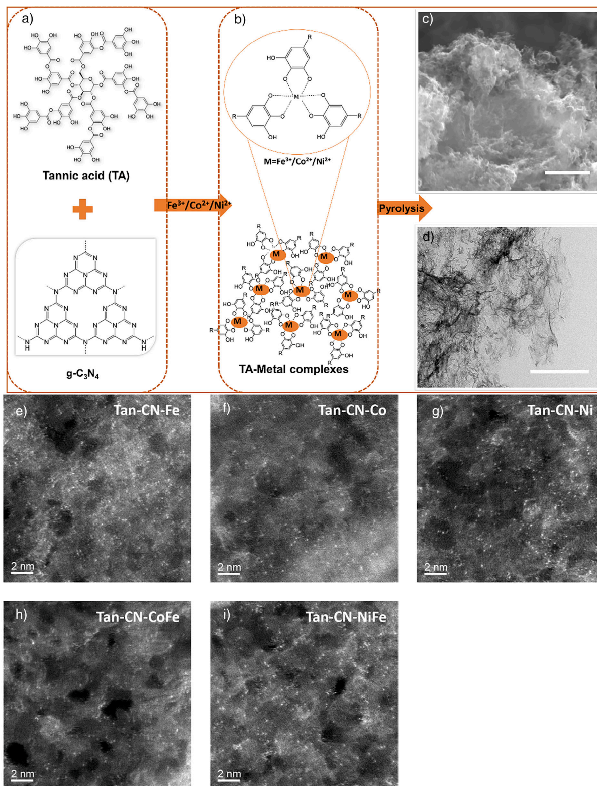
Figure 1. Scheme of the synthetic strategy of SACs. a) Molecular structures of tannic acid and g\text{-C}_3\text{N}_4 . b) \text{Fe}^{3+}/\text{Co}^{2+}/\text{Ni}^{2+} ions are coordinated with TA molecules. Morphological characterizations of the Tan-CN-Ni using c) scanning electron microscopy (SEM) and d) transmission electron microscopy (TEM) with the scale bar of 3 and 500 nm, respectively. HAADF-STEM images of e) Tan-CN-Fe, f) Tan-CN-Co, g) Tan-CN-Ni, h) Tan-CN-CoFe, and i) Tan-CN-NiFe with the scale bar of 2 nm.
