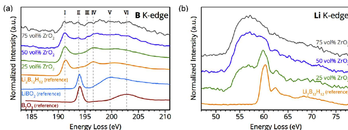
Figure 5. XRS spectra of reference compounds and different \text{Li}_2\text{B}_{12}\text{H}_{12} + \text{ZrO}_2 nanocomposites, corrected for the Zr \text{M}_{4,5} -edge contribution in the (a) boron K-edge region, and (b) Li K-edge region.
