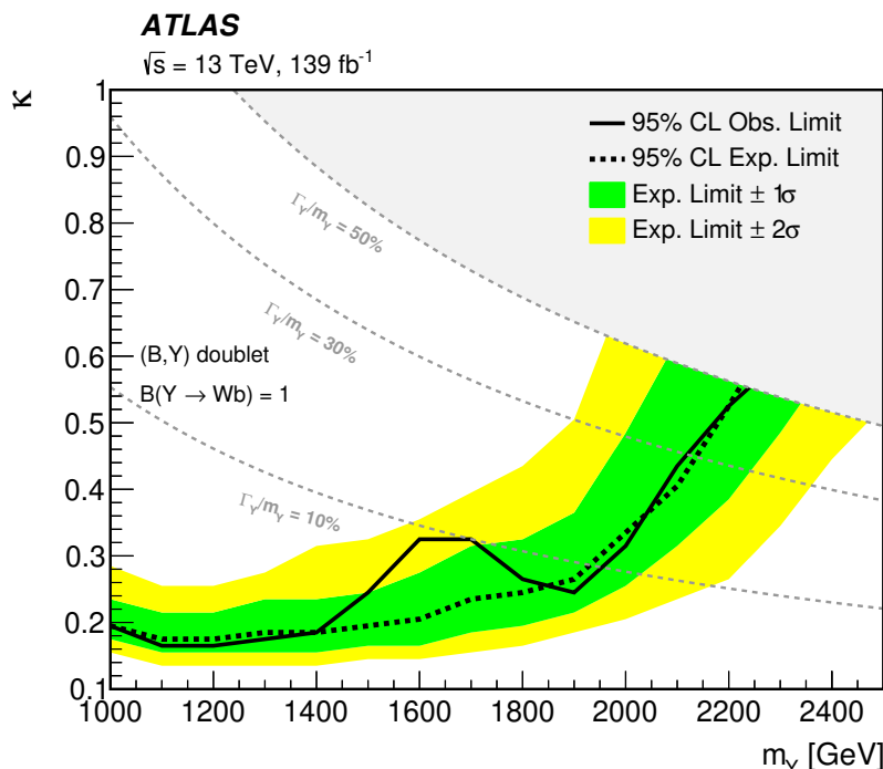
Figure 7. Observed (solid) and expected (dotted) 95% CL exclusion limits on the coupling constant \kappa as a function of the Y VLQ mass in the (B, Y) -doublet scenario. All \kappa values above the black contour lines are excluded at each mass point. The bands correspond to \pm 1 and \pm 2 standard deviations around the expected limit. Limits are only presented in the regime \Gamma_Y/m_Y \leq 50\% , where the theory calculations are known to be valid. The grey dotted isolines depict the highest (m, \kappa) values allowed for Y -doublet signals with various widths up to \Gamma_Y/m_Y = 50\% .
