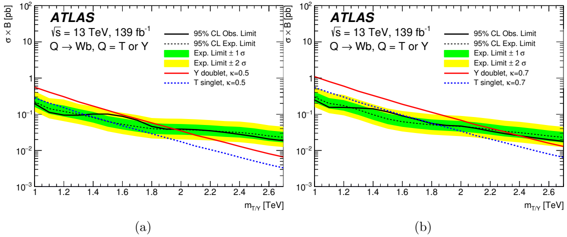
Figure 6. Expected (dotted) and observed (solid) cross-section limits times branching fraction for a Y VLQ in the (B, Y) doublet as a function of m_{T/Y} . Limits are computed for signals with couplings (a) \kappa = 0.5 and (b) \kappa = 0.7 . The branching fraction \mathcal{B}(Y \rightarrow Wb) is set to 1. The surrounding bands correspond to \pm 1 and \pm 2 standard deviations around the expected limit. The T -singlet quark's theoretical cross-section (corrected to NLO with the inclusion of finite-width effects) times branching fraction ( \mathcal{B}(T \rightarrow Wb) = 0.5 ) as a function of the T/Y mass is also shown (dashed blue line). The mass limit for a T singlet can then be obtained by computing the intersection of those cross-section limits and the T -singlet theory cross-section curve. The limits depend on \kappa because the natural width of the T/Y VLQ depends on \kappa .
