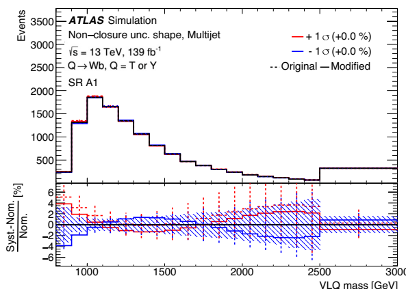
Figure 4. SR shape of the non-closure uncertainty on the multijet background estimation. The (solid) modified uncertainty is the smoothed version of the uncertainty that has been used in the likelihood fits and the original (dashed) uncertainty is the distribution before the smoothing procedure.
