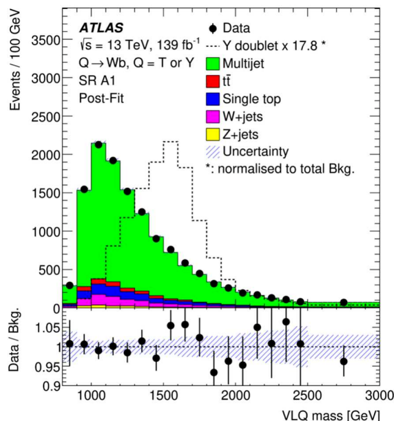
Figure 5. The post-fit distribution of m_{VLQ} in the SR A1 after the fit to data under the background-only hypothesis. All the uncertainties are included in this fit as nuisance parameters. The lower panel depicts the ratio of data to the fitted background yields. The hatched area in the lower panel represents the total uncertainty in the background, including the uncertainty in \mu^{\text{multijets}} . The overlaid dotted-line histogram in the upper panel shows the signal from a simulated Y VLQ with mass 1.6 TeV and \kappa = 0.5 , normalised to the total post-fit background yield.
