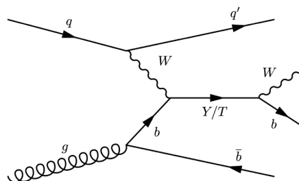
Figure 1. Leading-order Feynman diagram for the T/Y \rightarrow Wb process.
