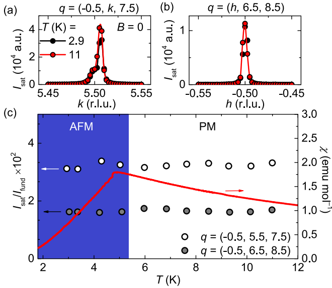
FIG. 5. CDW satellites across the antiferromagnetic transition. (a),(b) Reciprocal space profiles of (a) (-0.5, 5.5, 7.5) and (b) (-0.5, 6.5, 8.5) peaks at temperatures above and below T_N : at T = 11 K (red color) and T = 2.9 K (black), respectively. (c) Thermal dependence of these peaks' intensity normalized by the neighboring fundamental peaks (0, 5, 7) and (0, 6, 8) , respectively (white and gray points respectively; left-hand scale) at the vicinity of T_N at zero applied field. The temperature dependence of magnetic susceptibility \chi(T) measured at \mu_0 H = 0.01 T (red line; right-hand scale) illustrates the transition from a PM (white background) to AFM (blue background) state.
