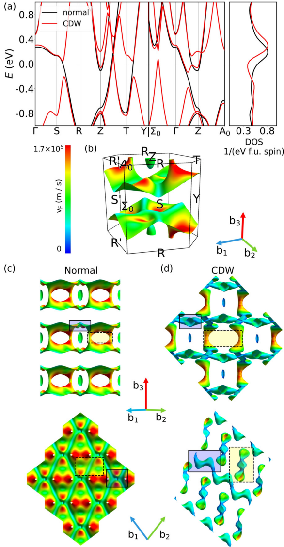
FIG. 3. (a) Electronic band structure and DOS of TmNiC 2 for both the normal phase (black line) and the q_{2c} -type CDW phase (red line). The Fermi energy is taken as zero. (b) The Fermi surface in the first Brillouin zone (FBZ) for the normal phase, along with the special points. (c) The Fermi surface for the normal phase from different perspectives (above, a lateral view; below, a top view). (d) Similarly, the Fermi surface for the q_{2c} -type CDW phase. The solid and dashed black boxes indicate the corresponding features in the Fermi surface of the two phases. The color scale represents the Fermi velocity. The high-symmetry \mathbf{k} points in the FBZ are \Gamma = (0, 0, 0) , S = (0, 0.5, 0) , R = (0, 0.5, 0.5) , Z = (0, 0, 0.5) , T = (-0.5, 0.5, 0.5) , Y = (-0.5, 0.5, 0) , \Sigma_0 = (0.39, 0.39, 0) , and A_0 = (0.39, 0.39, 0.5) .
