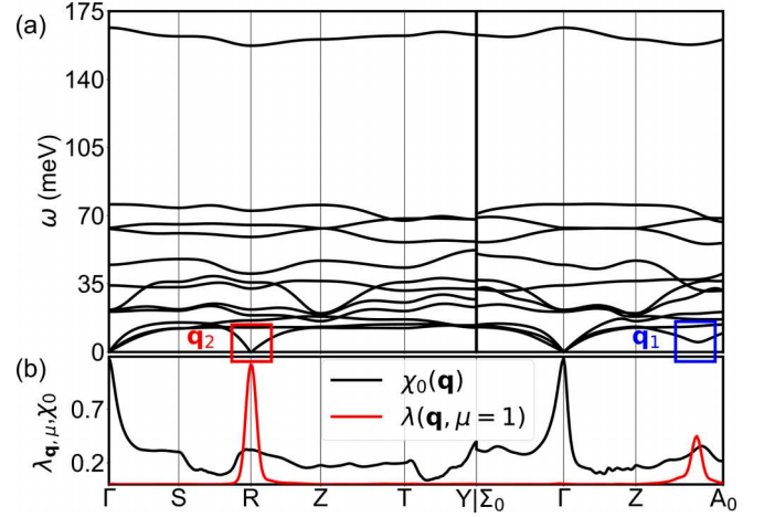
FIG. 4. (a) Phonon dispersion of TmNiC 2 revealing softening at the wave vectors q_2 and q_1 , highlighted as a red and blue box, respectively. (b) Electron-phonon coupling \lambda_{\mathbf{q},\mu} (red line) and nesting function \chi_0 (black line).
