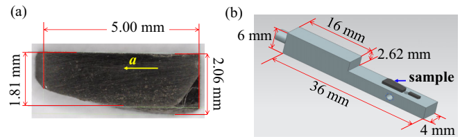
FIG. 1. (a) The \text{TmNiC}_2 sample used for the diffraction experiment. Dimensions and crystallographic a -axis direction are displayed. Sample thickness, not shown in the figure, is t = 0.66 mm. (b) Oxygen-free copper sample holder used for the synchrotron experiment with its key dimensions. The largest surface of the sample, parallel to the (011) plane, contacts the holder to maximize the heat exchange, and to ensure the mechanical stability of the sample exposed to strong magnetic field.
