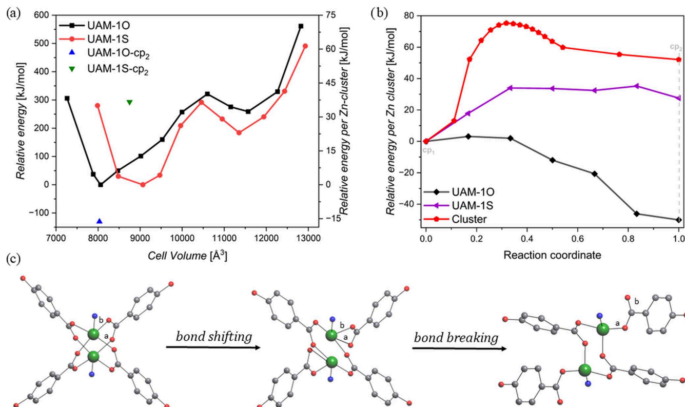
Figure 4. (a) Relative electronic energy. The values for both materials were calculated independently by subtracting from all values the value of minimum energy for a given \text{cp}_1 variant, without Zn–O bond breakage. (b) Energy profile calculated per single Zn-node for the transformation of the \text{cp}_1 to \text{cp}_2 configuration. Data for UAM-1O ( \text{Zn}_2(\text{oba})_2\text{TzTz} ) and UAM-1S ( \text{Zn}_2(\text{sba})_2\text{TzTz} ) were calculated using solid-state NEB, while data for cluster ( \text{Zn}_2\text{O}_4\text{N}_2 ) was calculated using NEB. NEB = nudged elastic band methodology. (c) Schematic representation of the considered transition mechanism. The initial structure \text{cp}_1 is presented on the left with two oxygens labeled as a and b, in the middle, the transition path with breaking both Zn–O(b) bond and the formation of new Zn–O(a) bond, and on the right are the resulting structures with different resulting nonbonded oxygens. Please note that \text{cp}_1 denotes the contracted phase of UAM-1S or UAM-1O, where the coordination number of zinc and the paddlewheel are preserved, while \text{cp}_2 refers to contracted phases with a decreed zinc coordination number to 4 and a disassembled paddlewheel. All calculations, except for cluster, were done for unit cell containing 16 Zn atoms.
