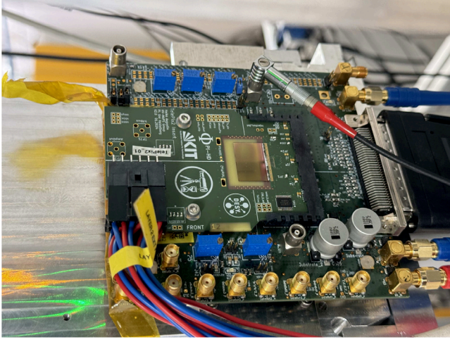
Fig. 3. Photograph of the TELEPIX2 chipboard, mounted to the motherboard. The red Lemo cable connects the fast hit-or, the Molex connector powers the chip, and the SCSI-III cable connects to the readout FPGA.
