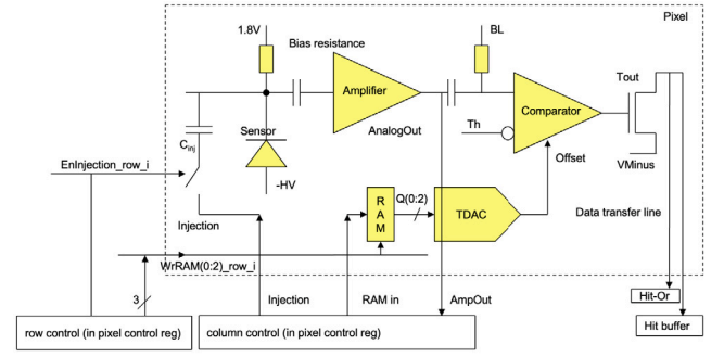
Fig. 2. Schematic drawing of the in-pixel functionality.
