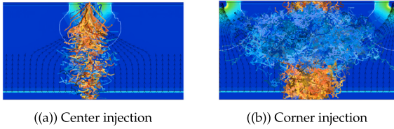
Fig. 5. Example of charge injection at the pixel center (a) and corner (b) at 1 ns for the Standard layout. The linegraphs are artificially overlapped with the electric field profile for visualization purposes. The electron and hole paths are represented in blue and orange, respectively.
