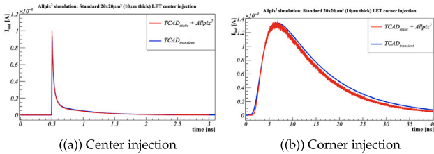
Fig. 6. Comparison of the induced current between TCAD and TCAD + Allpix 2 of a 20 \mu\text{m} \times 20 \mu\text{m} pixel in Standard layout. Plots show the injection in the center (a) and the corner (b) of the pixel.
