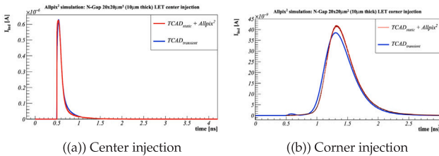
Fig. 7. Comparison of the induced current between pure TCAD and TCAD + Allpix 2 of a 20 \mu\text{m} \times 20 \mu\text{m} pixel in N-Gap layout. Plots show the injection in the center (a) and the corner (b) of the pixel.
