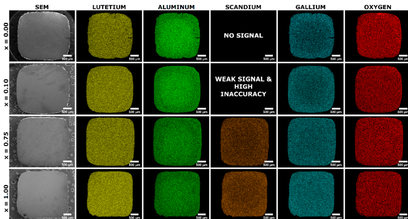
Figure 2. Multielemental EDS mapping of lutetium (Lu, yellow), aluminum (Al, green), scandium (Sc, orange), gallium (Ga, cyan), and oxygen (O, red) of \text{Pr}^{3+} -doped \text{Lu}_3\text{Al}_{2.5-x}\text{Sc}_x\text{Ga}_{2.5}\text{O}_{12} crystals, where x = 0.00, 0.10, 0.75 , and 1.00 .
