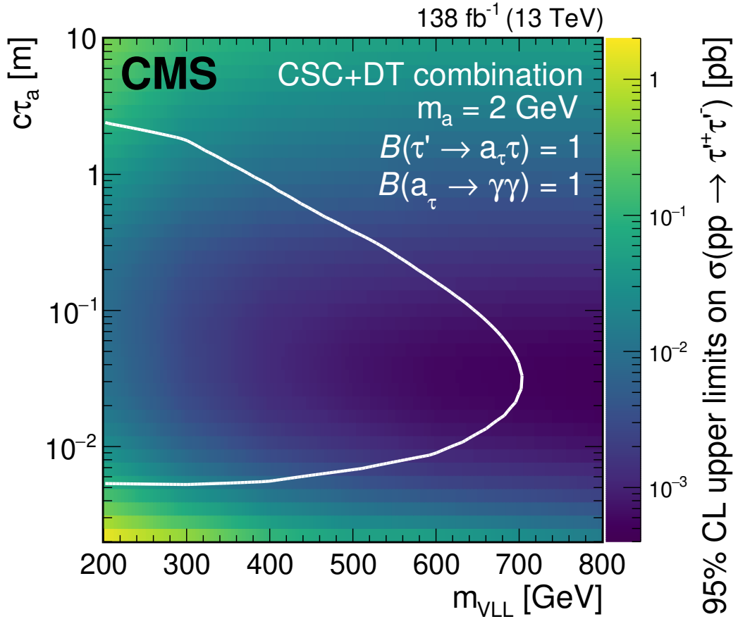
Figure 5: The 95% CL observed upper limits on the VLL production cross section as a function of the VLL mass and the pseudoscalar boson mean proper decay length c\tau_a . The pseudoscalar boson mass is 2 GeV. The area enclosed by the white line corresponds to the excluded region.
