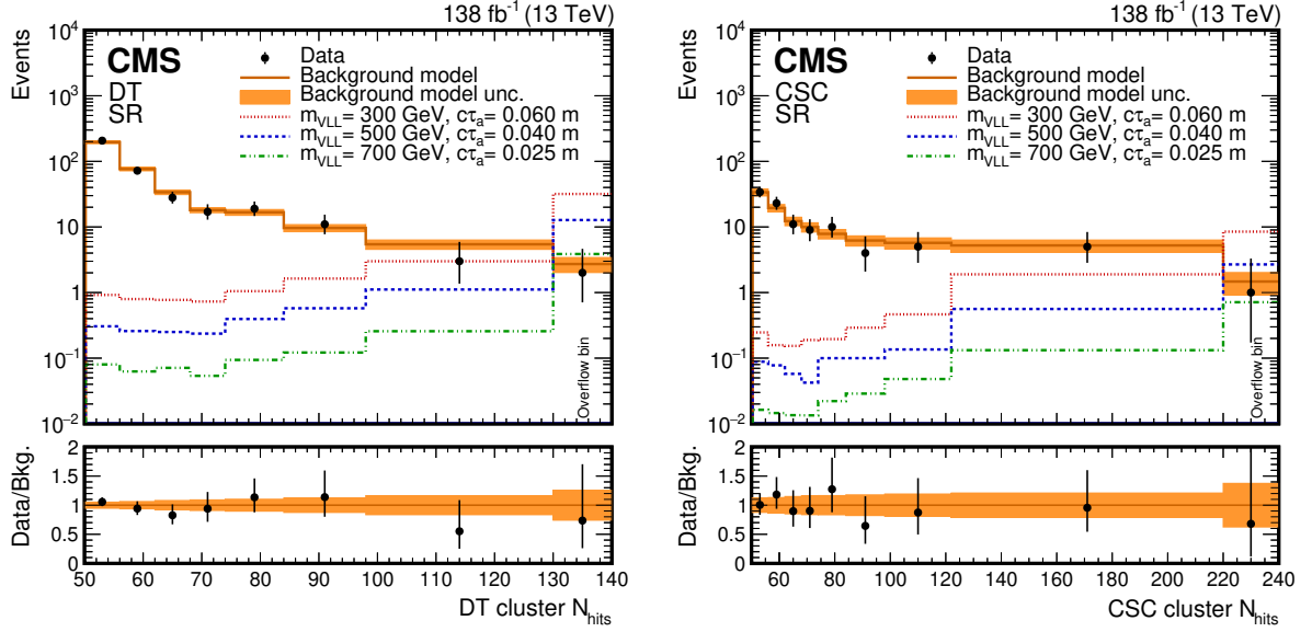
Figure 2: Distributions of the number of hits in the cluster ( N_{\text{hits}} ) for the DT (left) and CSC (right) cluster categories in the signal region (SR). The black markers represent the data. The solid orange line and associated orange band show the background prediction and corresponding uncertainty. The red dotted, blue dashed and green dashed-dotted lines denote different signal hypotheses for a pseudoscalar boson with a mass of 2 GeV. The last histogram bin contains all overflow events. The lower panel in each plot shows the ratio of the data to the estimated background.
