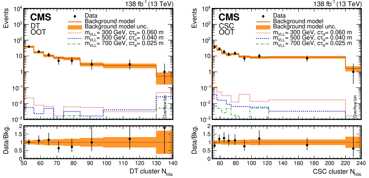
Figure 3: Distributions of the number of hits in the cluster ( N_{\text{hits}} ) for the DT (left) and CSC (right) cluster categories in the out-of-time (OOT) region. The black markers represent the data. The solid orange line and associated orange band show the background prediction and corresponding uncertainty. The red dotted, blue dashed and green dashed-dotted lines denote different signal hypotheses for a pseudoscalar boson with a mass of 2 GeV. The last histogram bin contains all overflow events. The lower panel in each plot shows the ratio of the data to the estimated background.
