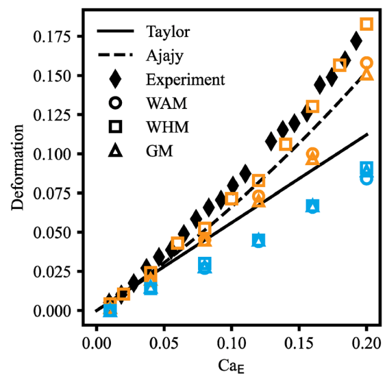
FIG. 8. Interpolation function comparison for the MSTF (blue markers) and CPF (orange markers) solvers. Experimental data are from Ha and Yang 70 and analytical solutions from Taylor 69 and Ajaji. 69
