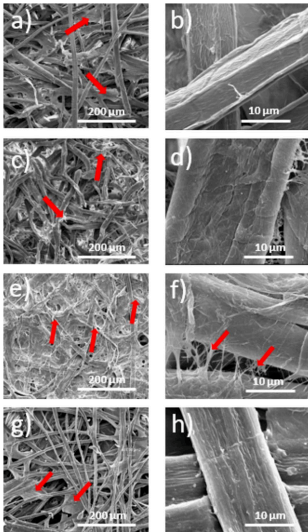
Fig. 6 Sample nr 2, Borussonetia fibers at 600 \times magnification showing regions of amorphous matter between the fibers (red arrows) (a), and at 10.000 \times magnification showing coarseness of the fiber (b). Sample nr 5, Gossypium fibers at 600 \times magnification, with visible ribbon-like twisting and regions of fibrillation (red arrows) (c), and at 10.000 \times magnification with visible flat and concave form of a single fiber (d). Sample nr 7, Cannabis sativa fibers at 600 \times and 10.000 \times magnification, showing high degree of fibrillation (red arrows) (e, f). Sample nr 25, Daphne fibers, at 600 \times and 10.000 \times magnification showing smooth surface and presence of inter-fiber amorphous matter (red arrows) (g, h)
