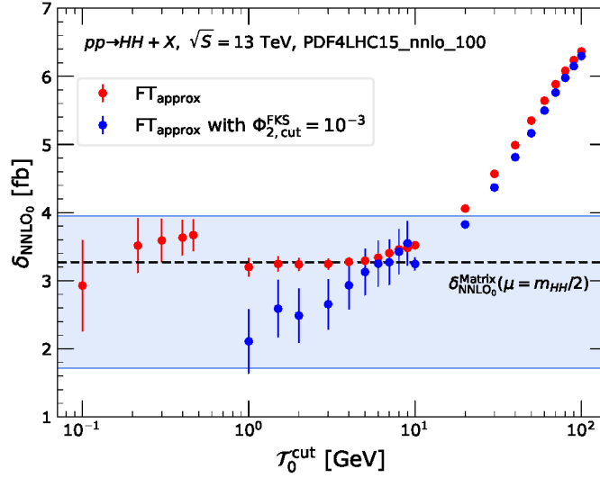
Figure 1: Relative NNLO corrections as a function of the slicing parameter \mathcal{T}_0^{\text{cut}} , evaluated at \sqrt{S} = 13 TeV and \mu = m_{HH}/2 , using the PDF4LHC15_nnlo_100 PDF set. The expected NNLO contribution from MATRIX, corresponding to 3.27 fb, is shown as a dashed black line.
