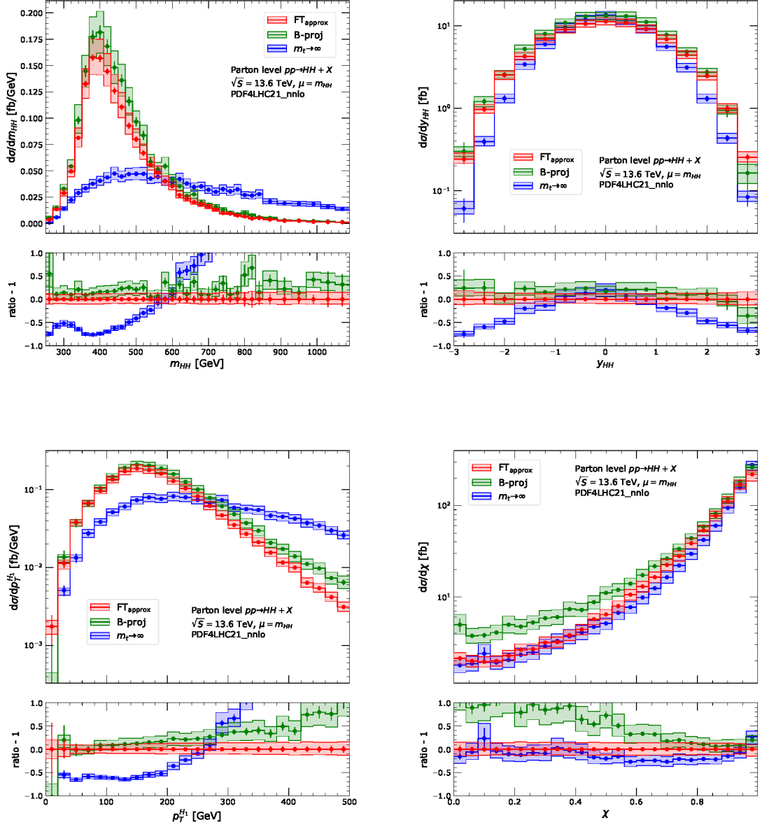
Figure 4: Comparison of partonic predictions obtained with the three top-quark mass approximations: m_t \rightarrow \infty (blue), B-proj (green) and FT_{\text{approx}} (red), shown for various differential distributions. These include the invariant mass of the Higgs boson pair ( m_{HH} , top-left), the rapidity of the pair ( y_{HH} , top-right), the transverse momentum of the hardest Higgs boson ( p_T^{H1} , bottom-left) and the \chi distribution (bottom-right). Results are obtained at \sqrt{S} = 13.6 TeV, with central scale \mu = m_{HH} , using PDF4LHC21_nnlo PDF set and 3-point scale variations.
