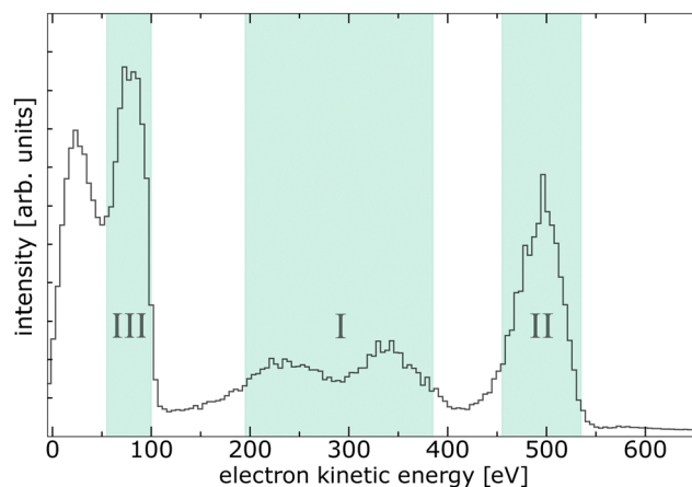
Fig. 3 Electron spectrum from all detected PEPIICO events of a mixed pyrimidine–water target at an exciting-photon energy of 620 eV. Three regions are indicated with electrons originating from different processes used as filter conditions for the ion–ion coincidence maps in Fig. 4(a)–(c).
