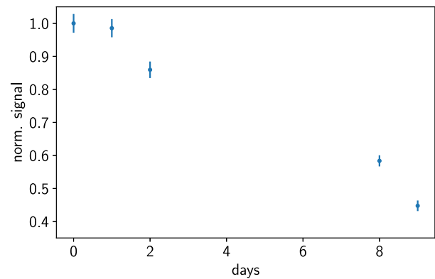
Fig. 7. The normalized signal amplitude from LED pulser measurements over time which indicates a degradation of the detector due to radiation.
