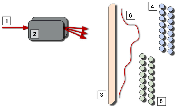
Fig. 5. Schematics of the EDS prototype setup at the FACET-II beamline. The 10 GeV electrons and scattered electrons from electron-laser interactions (1) are separated spatially with respect to their energy via a spectrometer dipole magnet (2), bent downwards and then detected by the EDS prototype in the scintillating screen (3), stainless-steel straws (4) and glass rods (5). As sketched in (6), a Compton spectrum is expected to be seen along the vertical axis.
