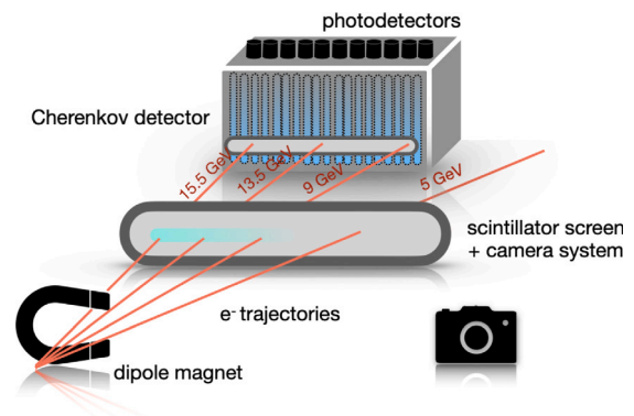
Fig. 3. Sketch of the Electron Detection System at LUXE behind a spectrometer dipole magnet. It shows the two complementary systems: the scintillating screen and camera system as well as the Cherenkov-based straw detector [5].
