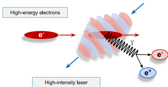
Fig. 1. Schematics of an electron bunch from the European XFEL interacting with a high-intensity laser pulse. A high-energy photon is created via the non-linear Compton effect and interacts further with the field to create a Breit-Wheeler electron-positron pair.
