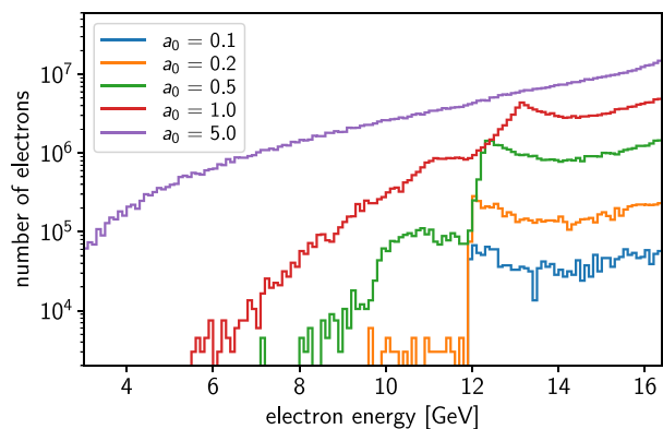
Fig. 2. Ptarmigan simulations of electron-laser collisions for different laser intensities a_0 . The number of scattered Compton electrons is given per bunch crossing with a bin size of 100 MeV. The blue line ( a_0 = 0.1 ) corresponds to the case of linear Compton scattering.
