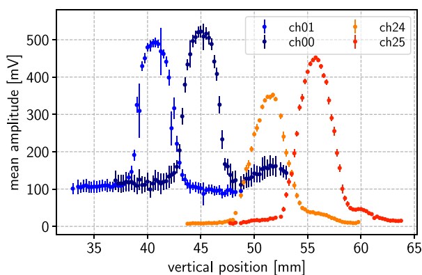
Fig. 6. Mean SiPM signal amplitudes of two air-filled steel straws (ch00 & ch01) and two glass rods (ch24 & ch25) as a function of the vertical detector position in the mono-energetic beam.
