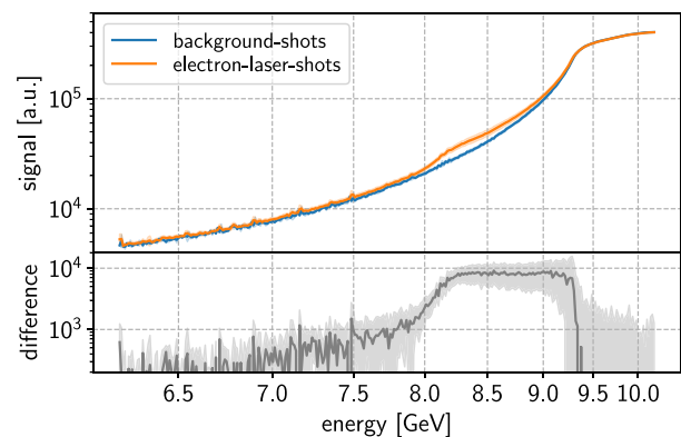
Fig. 8. Compton electron energy spectrum of electron-laser collisions in the E-320 experiment recorded with the screen detector. The signal (orange) and the background (blue) are averages over \mathcal{O}(10) shots with a 1\sigma band. The background signal is generated every 10 bunches, where no electron-laser collisions take place [3]. In gray the difference between the signal and the background is shown.
