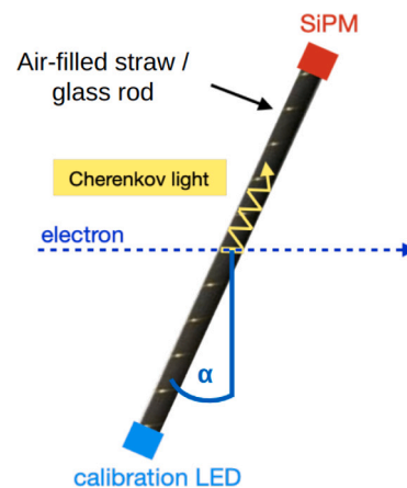
Fig. 4. Sketch of a straw in the straw detector. The Cherenkov light (yellow) created by the electron (blue arrow) is reflected towards the top of the straw and detected by a SiPM. Tilting the straws by an angle \alpha can be used to tune the sensitivity. [5].
