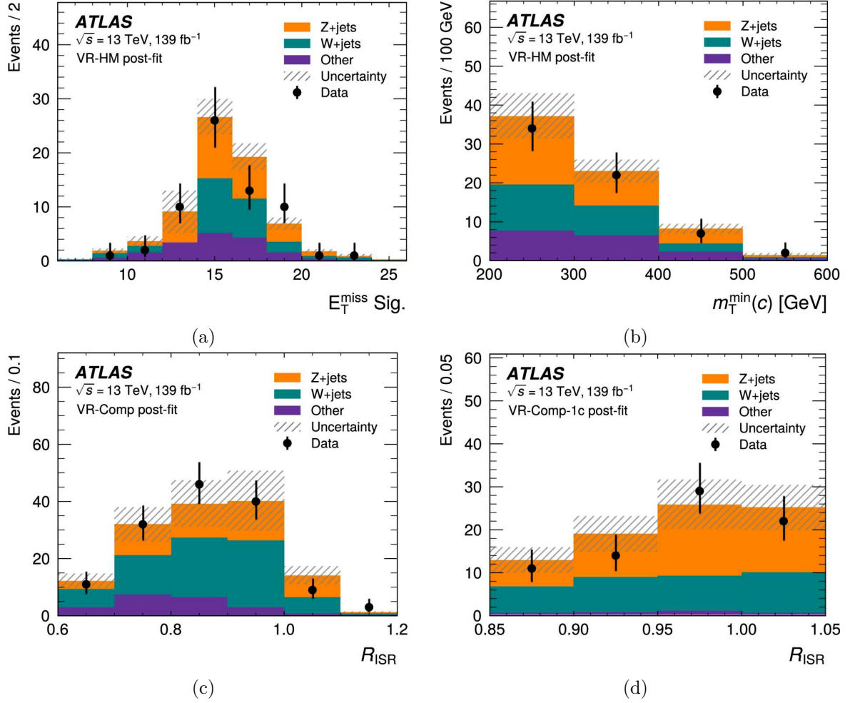
Figure 5. Distributions, in various validation regions, showing the level of agreement between the data (points) and the SM expectation (stacked histograms, after simultaneously fitting the Z +jets and W +jets backgrounds) for variables which have different selection criteria in the signal regions: (a) E_T^{\text{miss}} \text{ Sig.} in VR-HM, (b) m_T^{\text{min}}(c) in VR-HM, (c) R_{\text{ISR}} in VR-Comp, and (d) R_{\text{ISR}} in VR-Comp-1c. The hatched uncertainty band around the total SM expectation includes theory-based and detector-related systematic uncertainties and MC statistical uncertainties. Processes with top quarks and multiple vector bosons are included in “Other”. The right-most bin in each histogram does not include the overflow entry but the x -axis range is chosen to include all observed data.
