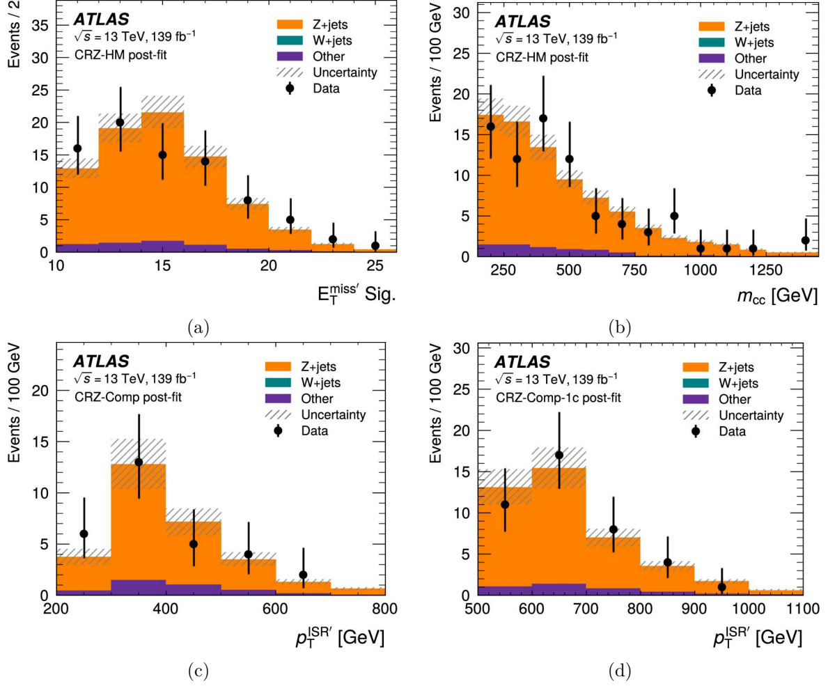
Figure 3. Distributions showing the level of agreement between data (points) and the SM expectation (stacked histograms, after simultaneously fitting the Z +jets and W +jets backgrounds) in the Z +jets control regions for some variables which have different selection criteria in the signal regions: (a) E_T^{\text{miss}} \text{ Sig.} in CRZ-HM, (b) m_{cc} in CRZ-HM, (c) p_T^{\text{ISR}'} in CRZ-Comp, and (d) p_T^{\text{ISR}'} in CRZ-Comp-1c. The hatched uncertainty band around the total SM expectation includes theory-based and detector-related systematic uncertainties and MC statistical uncertainties. Processes with top quarks and multiple vector bosons are included in “Other”. The W +jets background contribution is negligible and not visible in the plots. The right-most bin in each histogram does not include the overflow entry but the x -axis range is chosen to include all observed data.
