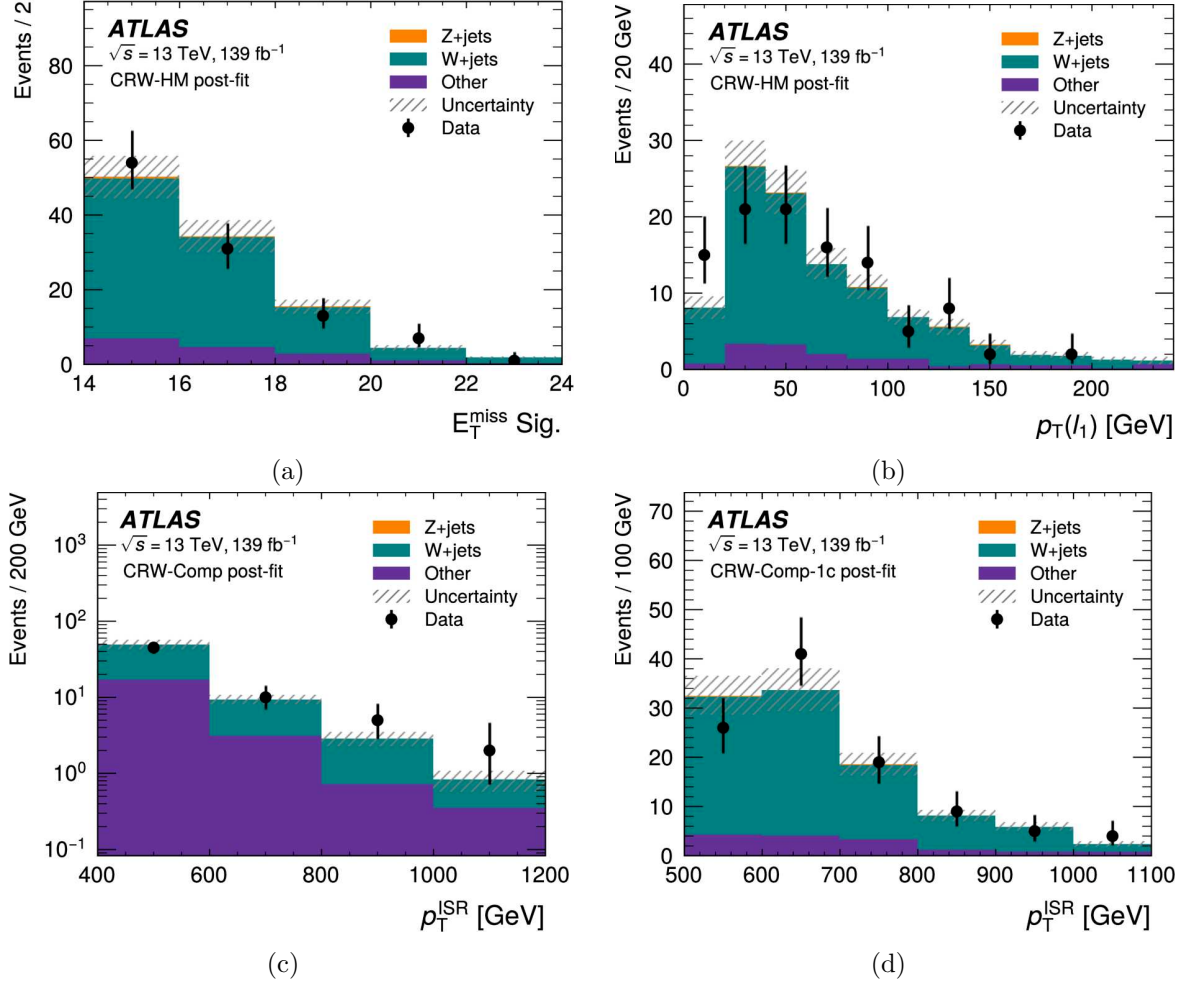
Figure 4. Distributions showing the level of agreement between the data (points) and the SM expectation (stacked histograms, after simultaneously fitting the Z+jets and W+jets backgrounds) in the W+jets control regions for some variables which have different selection criteria in the signal regions: (a) E_T^{\text{miss}} \text{ Sig.} in CRW-HM, (b) p_T of leading lepton in CRW-HM, (c) p_T^{\text{ISR}} in CRW-Comp, and (d) p_T^{\text{ISR}} in CRW-Comp-1c. The hatched uncertainty band around the total SM expectation includes theory-based and detector-related systematic uncertainties and MC statistical uncertainties. Processes with top quarks and multiple vector bosons are included in “Other”. The Z+jets background contribution is negligible and not visible in the plots. The right-most bin in each histogram does not include the overflow entry but the x -axis range is chosen to include all observed data.
