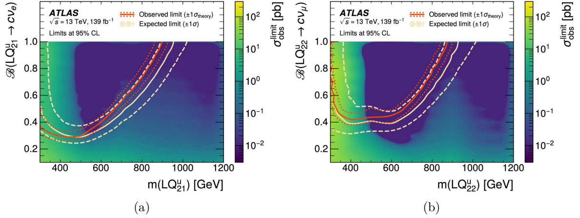
Figure 10. Expected (white) and observed (red) exclusion limits at 95% CL for up-type scalar LQs coupled to (a) first- and (b) second-generation leptons. The observed upper limit on the production cross-section is plotted on the z -axis as a function of (a) \mathcal{B}(\text{LQ}^{\text{u}} \rightarrow c\nu_e) with the alternative decay being \text{LQ}^{\text{u}} \rightarrow s + e and (b) \mathcal{B}(\text{LQ}^{\text{u}} \rightarrow c\nu_\mu) with the alternative decay being \text{LQ}^{\text{u}} \rightarrow s + \mu ( y -axis) and the leptoquark masses ( x -axis). The branching fractions above and masses below the lines (high branching fraction and low mass, and thus high production cross-section) are excluded. The \pm 1\sigma interval of the expected limit is shown as dashed white lines while the effect of varying the signal cross-section by \pm 1\sigma of its predicted theoretical uncertainty is shown as red dashed lines.
