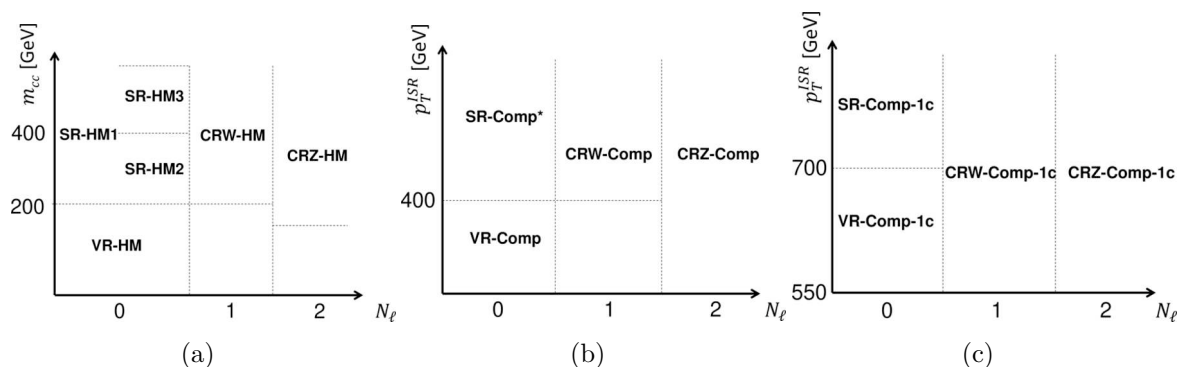
Figure 2. Phase-space partitioning between the signal, control, and validation regions for the (a) High-Mass signal regions, (b) Compressed signal regions SR-Comp1, SR-Comp2 and SR-Comp3, and (c) SR-Comp-1c. Control regions differ from the signal and validation regions by the electron and muon multiplicities (exactly one electron or muon in the W +jets control regions and two electrons or muons in the Z +jets regions) while the validation regions veto events with leptons as in the signal regions. The asterisk in “SR-Comp*” is a wildcard character to denote all the Compressed signal regions which require two c -tagged jets.
