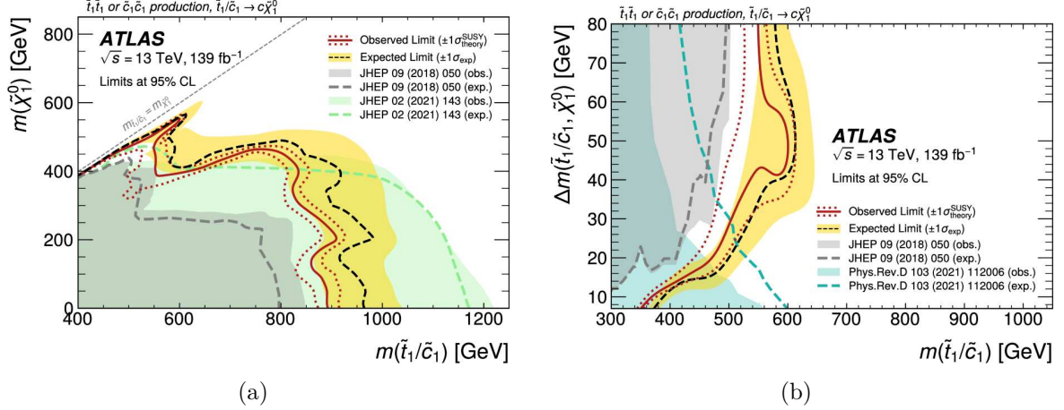
Figure 8. Exclusion limits at 95% CL for pair production of top squarks decaying into charm quarks and neutralinos. The expected limit is shown as a dashed line while the \pm 1\sigma interval is shown as a yellow band. The observed limit is shown as a red line and the effect of varying the signal cross-section by \pm 1\sigma of its predicted theoretical uncertainty is shown as red dashed lines. The contours are shown as two-dimensional projections for masses of squarks and neutralinos (a) and their differences (b). The exclusion contour from the previous ATLAS result that used charm tagging (ref. [30]) is shown as a grey-dashed line (expected) and grey-filled contour (observed). For (a), the single-squark-production exclusion contour from the ATLAS squarks and gluinos search that did not utilize charm tagging (ref. [33]) is shown as a green-dashed line (expected) and green-filled contour (observed), while for (b), the contour from the ATLAS single-jet search (ref. [32]) is shown as a cyan-dashed line (expected) and cyan-filled contour (observed).
