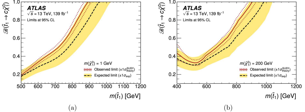
Figure 9. The expected and observed exclusion contours for pair production of top squarks decaying into top or charm quarks and neutralinos. The contours are shown as two-dimensional projections in the plane of the squark mass and assumed branching fraction, whose value is varied between 0 (all decays to t + \tilde{\chi}_1^0 ) and 1 (all decays to c + \tilde{\chi}_1^0 ). The mass of the neutralino is fixed to either (a) 1 GeV or (b) 200 GeV. The cross-section limits for the contours are calculated by combining the signal regions as discussed earlier in the paper. The branching fractions above and masses below the lines (high branching fraction and low mass, and thus high production cross-section) are excluded. The expected limit is shown as a dashed line, while the \pm 1\sigma interval is shown as a yellow band. The observed limit is shown as a red line and the effect of varying the signal cross-section by \pm 1\sigma of its predicted theoretical uncertainty is shown as red dashed lines.
