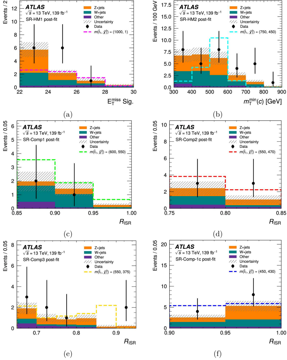
Figure 7. Distributions for the signal regions showing the data (points) and the expected backgrounds (stacked histograms), after simultaneously fitting all the control regions. The histograms are binned in the key variables for each signal region: (a) E_T^{\text{miss}} \text{ Sig.} for SR-HM1, (b) m_T^{\text{min}}(c) for SR-HM2, (c) R_{\text{ISR}} for SR-Comp1, (d) R_{\text{ISR}} for SR-Comp2, (e) R_{\text{ISR}} for SR-Comp3, and (f) R_{\text{ISR}} for SR-Comp-1c. The hatched band is the total systematic uncertainty for the expected backgrounds. Distributions of representative \tilde{t}_1 \bar{\tilde{t}}_1 signals for different mass assumptions (or similar) are shown as dashed lines using pre-fit signal contributions. Processes with top quarks and multiple vector bosons are included in “Other”. The right-most bin in each histogram does not include the overflow entry but the x -axis range is chosen to include all observed data.
