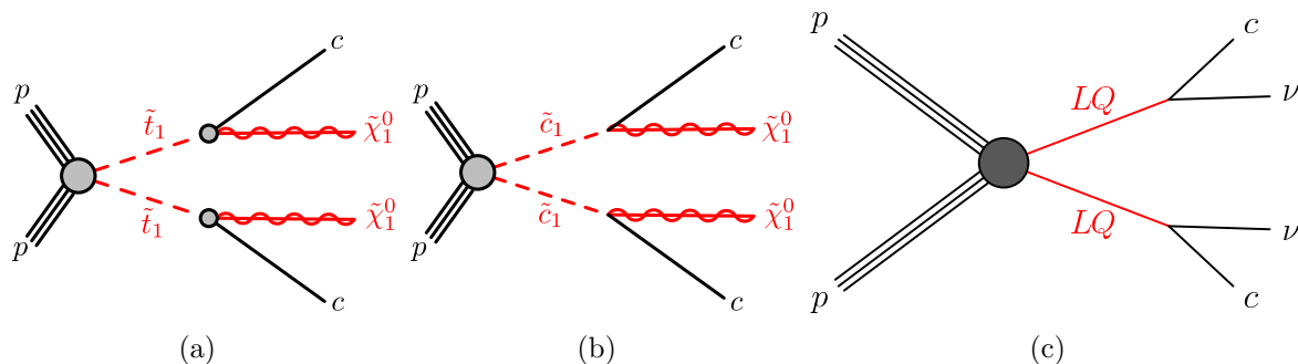
Figure 1. Representative diagrams for pair production of (a) top squarks ( \tilde{t}_1 ) and (b) charm squarks ( \tilde{c}_1 ), with subsequent decay into charm quarks and neutralinos ( \tilde{\chi}_1^0 ), and (c) pair production of leptoquarks decaying into charm quarks and neutrinos.
