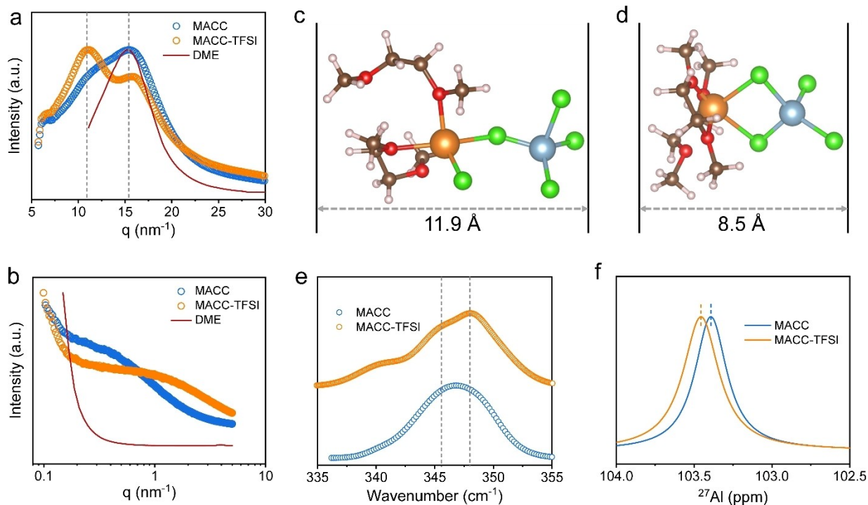
Figure 4. Electrolyte characterizations. a) WAXS and b) SAXS profiles of MACC and MACC-TFSI. Representative \text{AlCl}_4^- -containing clusters in c) MACC and d) MACC-TFSI derived from the snapshots through AIMD simulations. e) Raman and f) ^{27}\text{Al} NMR spectra of MACC and MACC-TFSI.
