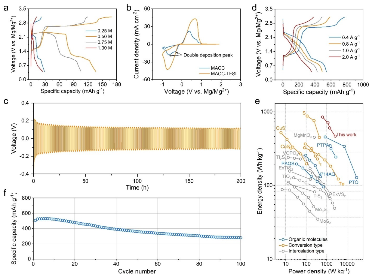
Figure 2. Electrochemical performance of the Mg//Te dual-ion battery. a) GCD curves of Mg//Te cells in the MACC electrolytes added with different concentrations of \text{Mg}(\text{TFSI})_2 . Pristine glass fiber separators were used. b) CV curves obtained from Mg//Pt cells using the MACC and MACC-TFSI electrolytes at a scan rate of 25 \text{ mVs}^{-1} . c) Galvanostatic Mg stripping/plating in Mg//Mg symmetric cells with the MACC-TFSI electrolyte at 0.1 \text{ mAcm}^{-2} and 0.1 \text{ mAhcm}^{-2} . d) GCD curves of the Mg//Te cell with the MACC-TFSI electrolyte at various current densities. A GO-covered glass fiber separator was used. e) Ragone plots presenting the energy density and power density of the Te electrode in comparison with recently reported Mg battery cathodes. All the calculations are based on the mass of active cathode materials. f) Cycling performance of the Mg//Te cell using the MACC-TFSI electrolyte at 2.0 \text{ A g}_{\text{Te}}^{-1} .
