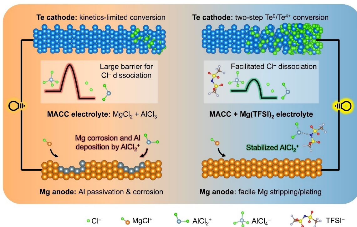
Figure 1. Schematic illustration of Mg//Te cells with the MACC electrolyte (left) and the MACC-TFSI electrolyte (right).
