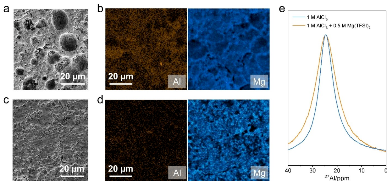
Figure 5. Analysis of Mg anode in Mg//Te dual-ion cell. a) SEM image and b) EDX elemental mapping (Al, Mg) of the Mg anode surface from Mg//Te cell with MACC electrolyte after 10 charge/discharge cycles at 200 \text{ mA g}_{\text{Te}}^{-1} . c) SEM image and d) EDX elemental mapping (Al, Mg) of the Mg anode surface from Mg//Te cell with MACC-TFSI electrolyte after 10 charge/discharge cycles at 200 \text{ mA g}_{\text{Te}}^{-1} . e) ^{27}\text{Al} NMR spectra of 1 M \text{AlCl}_3 in diglyme and 1 M \text{AlCl}_3 + 0.5 \text{ M Mg}(\text{TFSI})_2 in diglyme.
