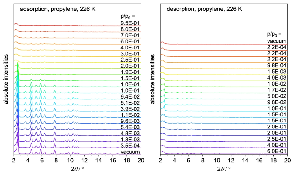
Figure 4. In situ PXRD patterns ( \lambda = 0.15405 nm) along with the adsorption (left) and desorption (right) of propylene at 226 K.
