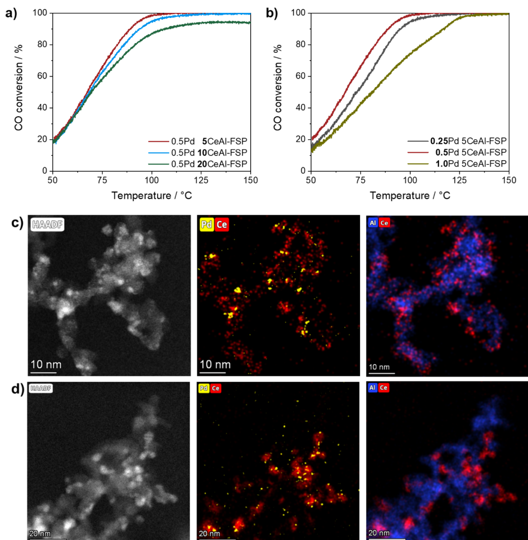
Figure 5. Catalytic activity results in terms of CO conversion of the FSP-synthesized Pd/CeO 2 –Al 2 O 3 catalysts during CO oxidation reaction (1000 ppm CO/8% O 2 /N 2 ) after a degreening run showing the influence of CeO 2 (a) and Pd loading (b) (in all cases normalized to Pd amount, cf. experimental) on the catalytic performance. HAADF-STEM images with the corresponding EDXS mappings of 1.0Pd 5CeAl-FSP (c) and 0.5Pd 20CeAl-FSP (d).
