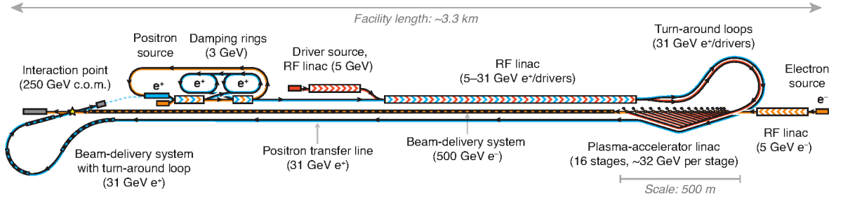
Figure 1.3: Schematic of the proposed HALHF collider. The positron bunches (blue) are produced and radiatively dampened and then accelerated together with electron drive bunches (red). After the turnaround, the drive bunches are used to accelerate an electron bunch (orange) in plasma stages, and the positrons are transferred to the interaction point at the other end. Image from Ref. [30] (CC-BY 4.0).
