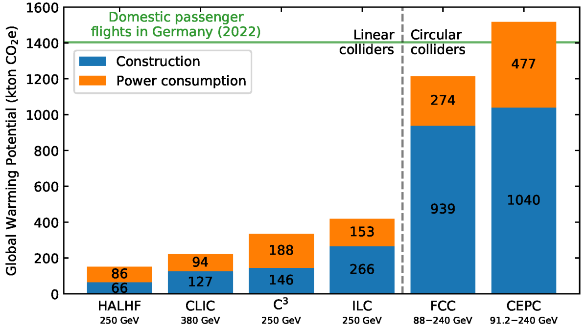
Figure 1.4: GWP from different colliders over their planned operational lifetime, with emissions from construction in blue and from power consumption in orange. The linear and circular colliders are separated by the vertical dashed line. The center-of-mass energy included for this estimation is noted below the name of each design. Note that for the C 3 design, energy-saving schemes reducing the power consumption by 44% were proposed [40]. Also note that this is a comparison of Higgs factories, and higher center-of-mass energies for other physics cases are considered in some designs, e.g. FCC and CEPC. As a reference, the GWP from German domestic passenger flights in 2022 is shown with the horizontal green line [43]. This Figure is an adaptation from Ref. [40] (CC-BY 4.0), with the HALHF GWP estimated as described in the text.
